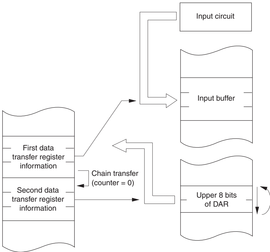
Figure 9.13 Chain Transfer when Counter = 0
