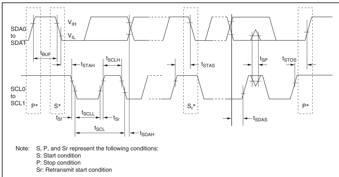
Figure 26.47 I²C Bus Interface 2 Input/Output Timing (Option)
