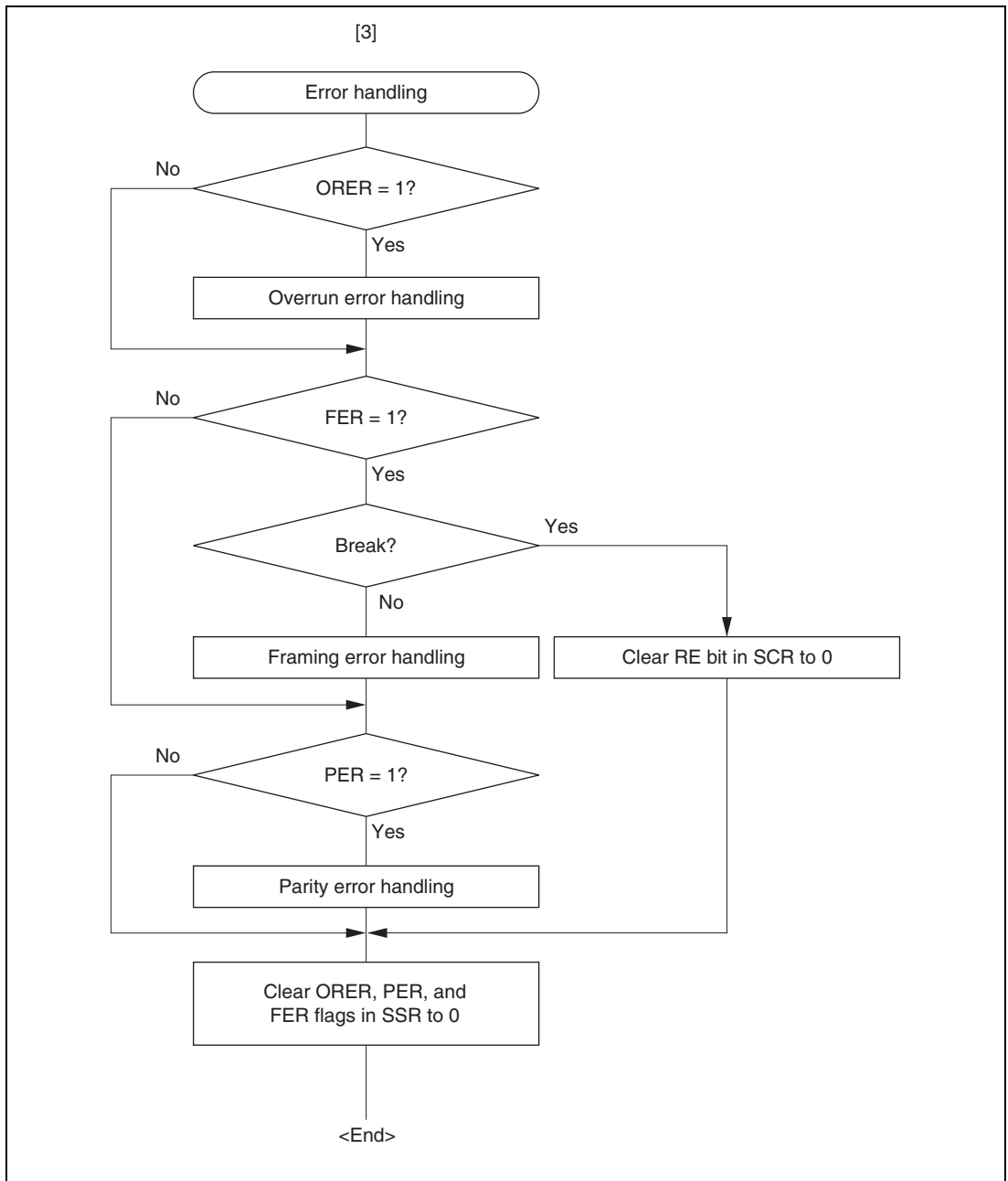
Figure 15.9 Sample Serial Reception Data Flowchart (2)
