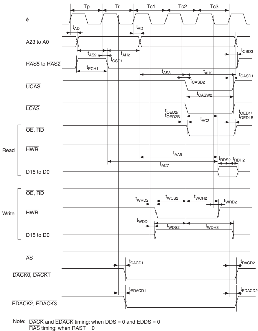
Figure 26.18 DRAM Access Timing: Three-State Access (RAST = 1)
