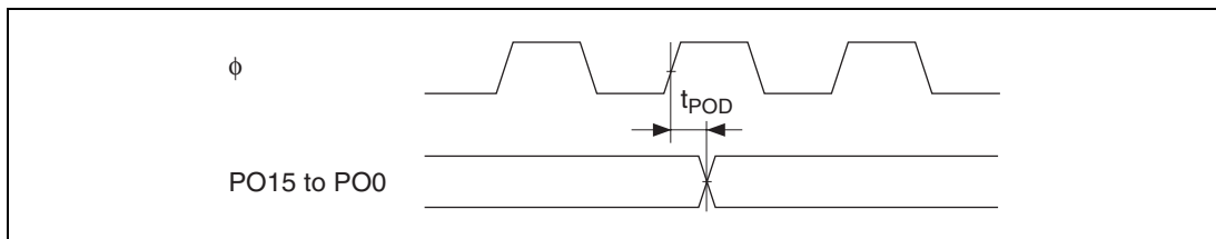
Figure 26.37 PPG Output Timing
