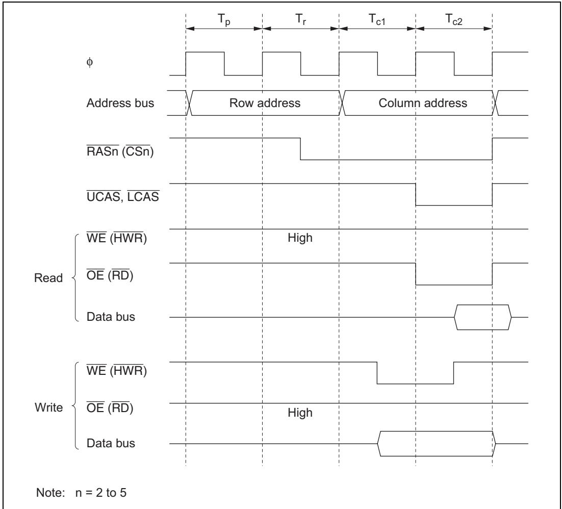
Figure 6.33 DRAM Basic Access Timing (RAST = 0, CAST = 0)
