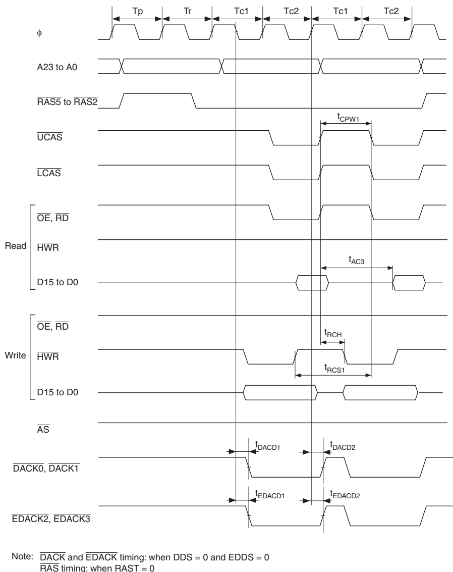
Figure 26.17 DRAM Access Timing: Two-State Burst Access
