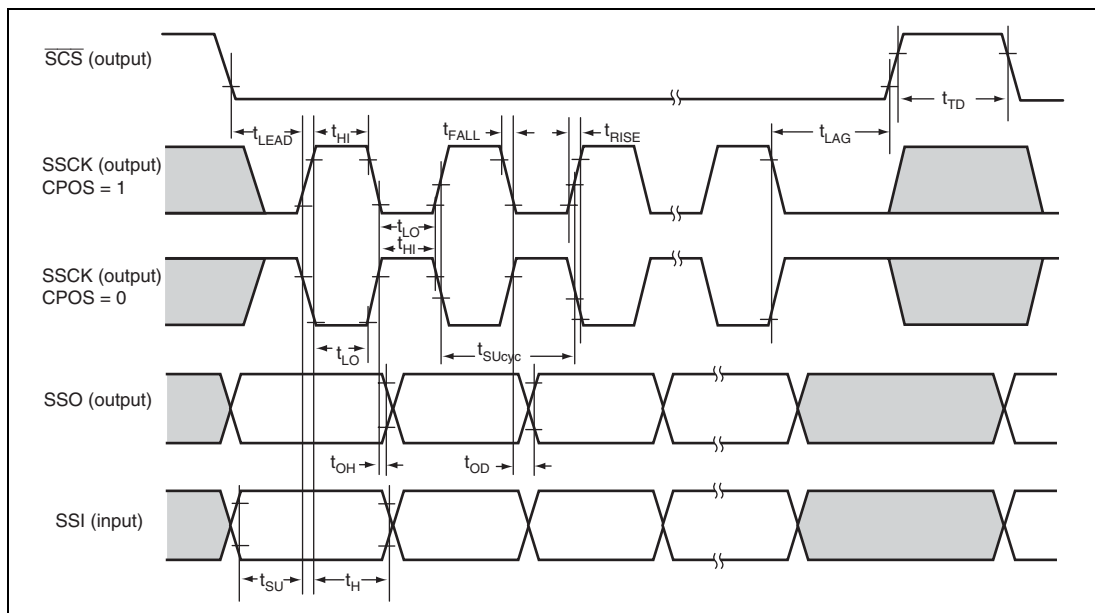
Figure 26.49 SSU Timing (Master, CPHS = 1)
