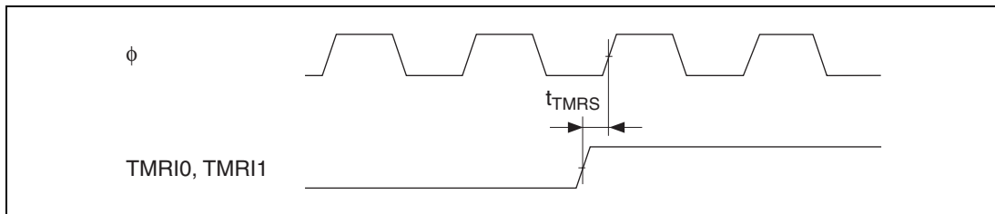
Figure 26.42 8-Bit Timer Reset Input Timing
