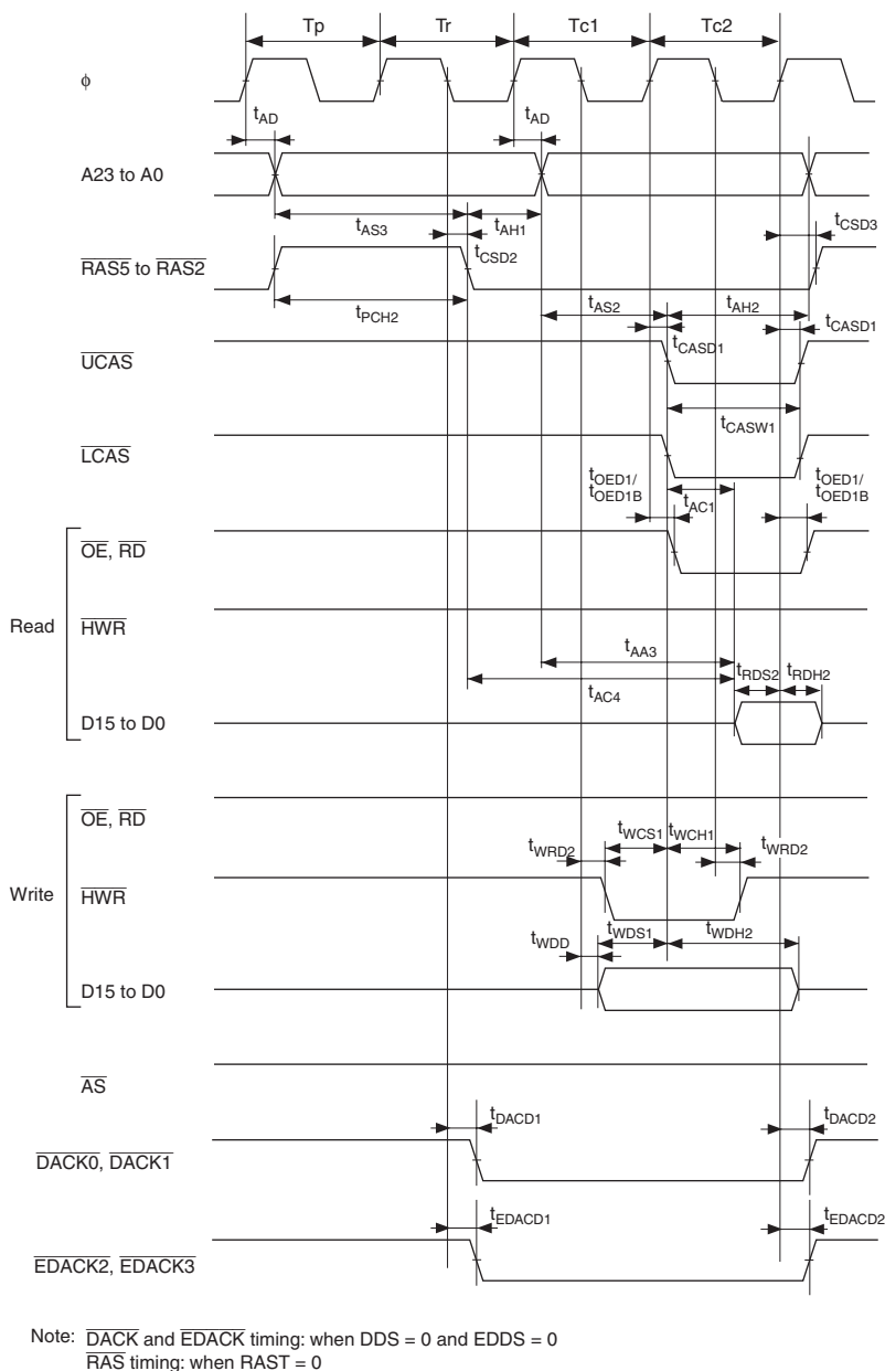
Figure 26.15 DRAM Access Timing: Two-State Access
