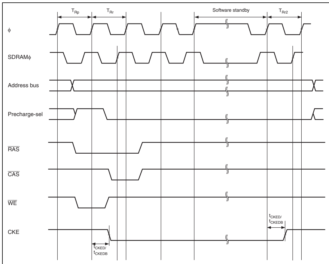
Figure 26.27 Synchronous DRAM Self-Refresh Timing
