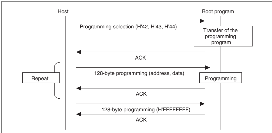
Figure 21.12 Programming Sequence
