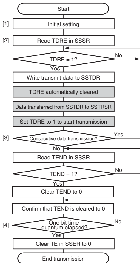
Figure 19.14 Flowchart Example of Transmission Operation (Clock Synchronous Communication Mode)
