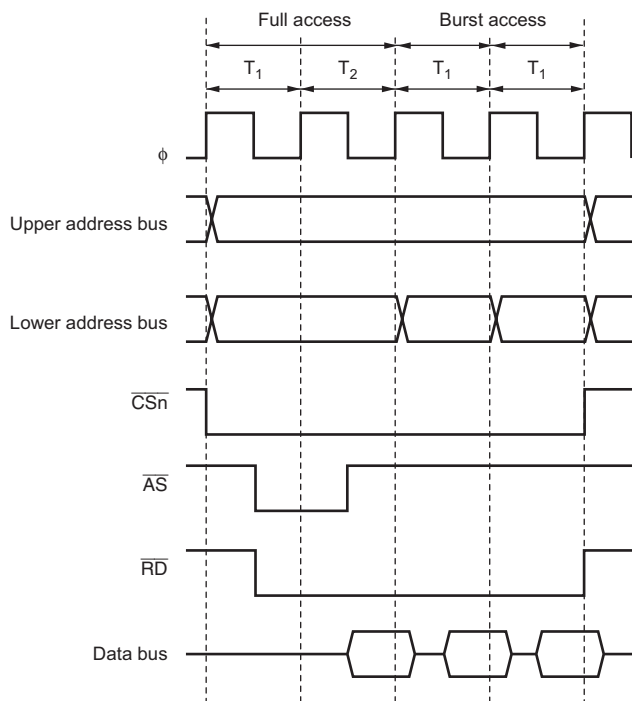
Figure 6.76 Example of Burst ROM Access Timing (ASTn = 0, 1-State Burst Cycle)
