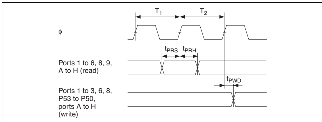
Figure 26.36 I/O Port Input/Output Timing
