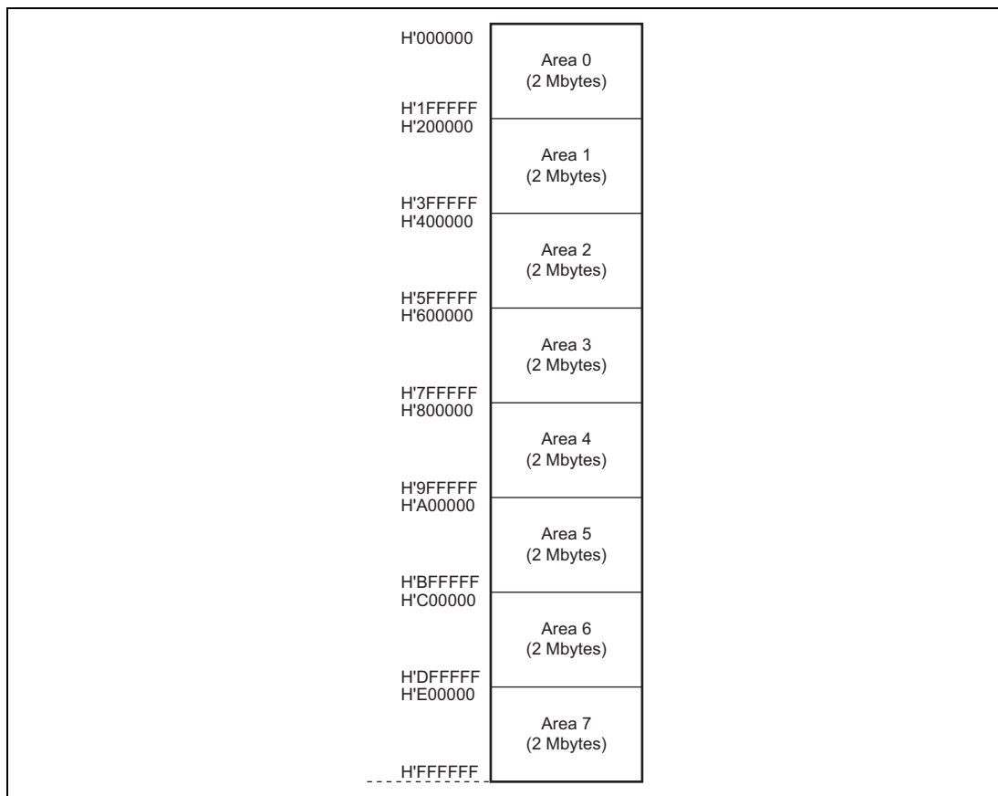
Figure 6.6 Area Divisions
