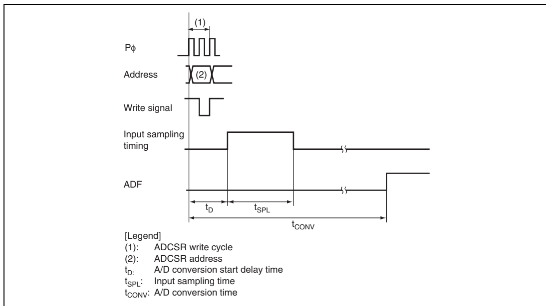
Figure 17.6 A/D Conversion Timing
