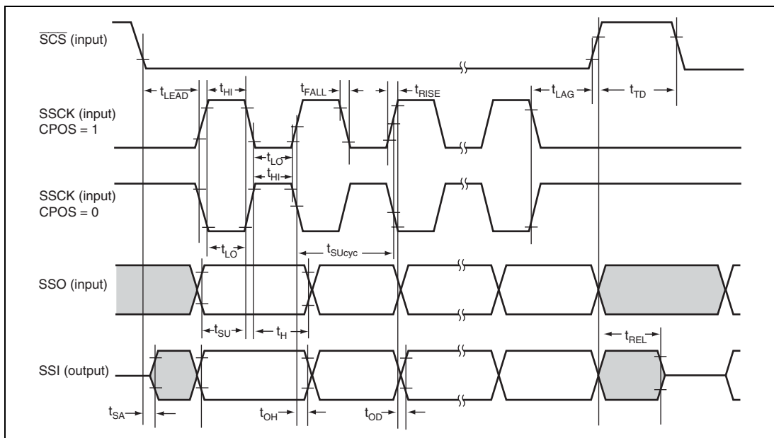
Figure 26.52 SSU Timing (Slave, CPHS = 0)
