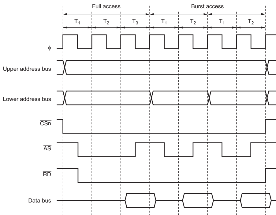
Figure 6.75 Example of Burst ROM Access Timing (ASTn = 1, 2-State Burst Cycle)
