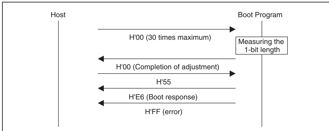
Figure 21.9 Bit-Rate-Adjustment Sequence
