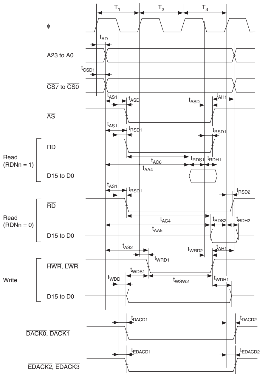
Figure 26.9 Basic Bus Timing: Three-State Access
