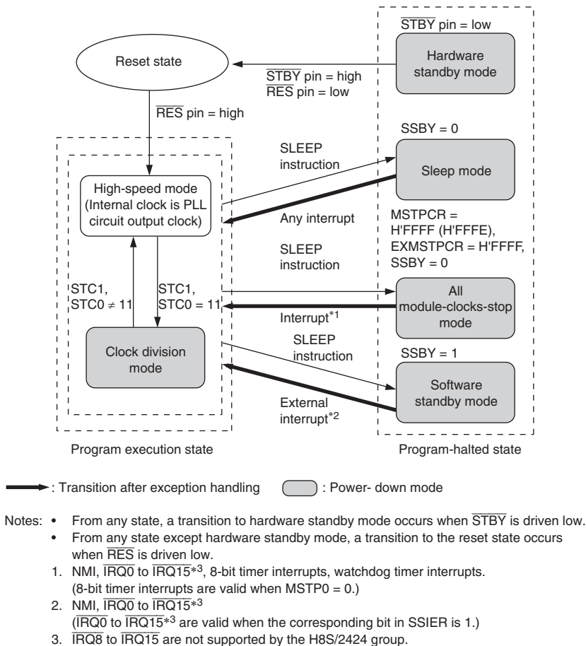
Figure 24.1 Mode Transitions
