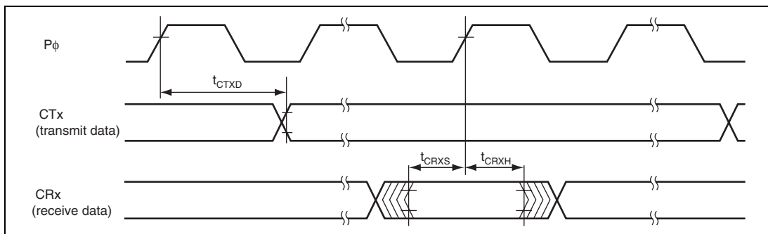
Figure 26.48 RCAN-ET Input/Output Timing
