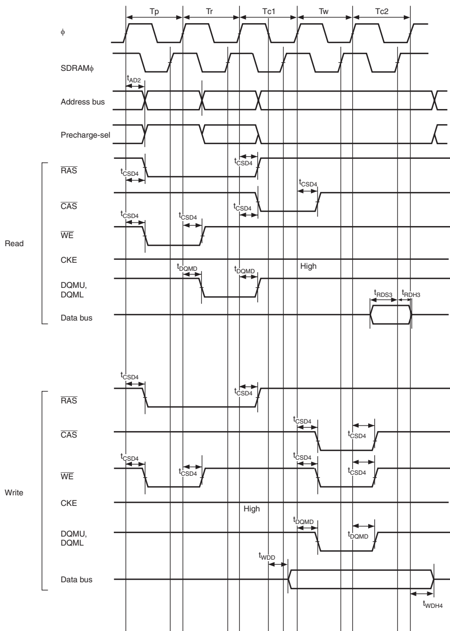
Figure 26.26 Synchronous DRAM Basic Access Timing (CAS Latency 2)
