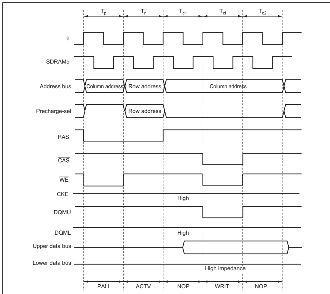
Figure 6.61 DQMU and DQML Control Timing (Upper Byte Write Access: \text{SDWCD} = 0 , CAS Latency 2)
