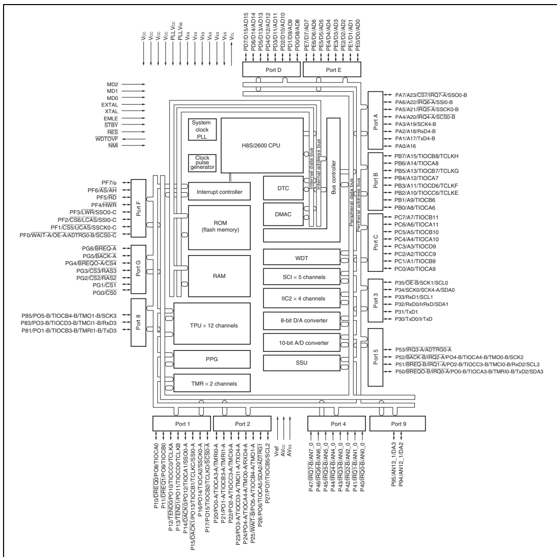
Figure 1.3 Block Diagram of H8S/2424 Group
