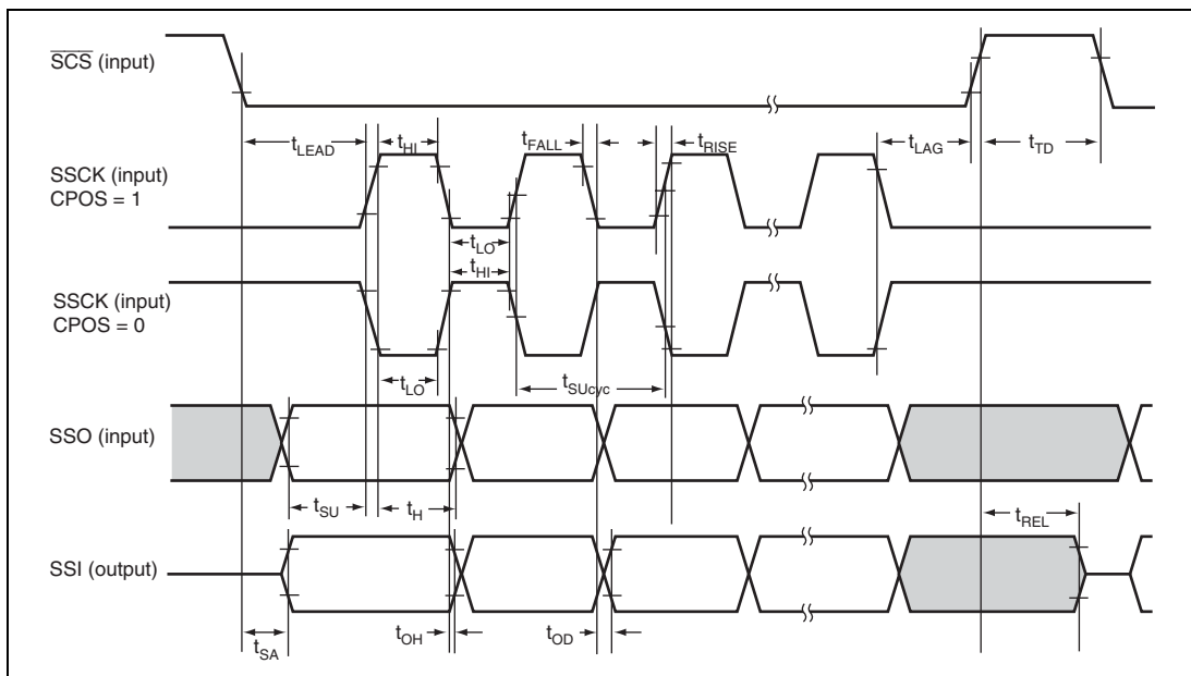
Figure 26.51 SSU Timing (Slave, CPHS = 1)
