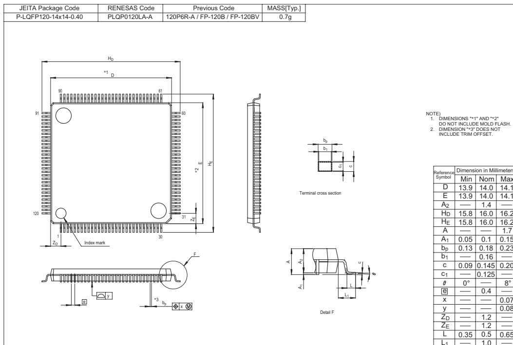
Figure C.3 Package Dimensions (LQFP1414-120)
