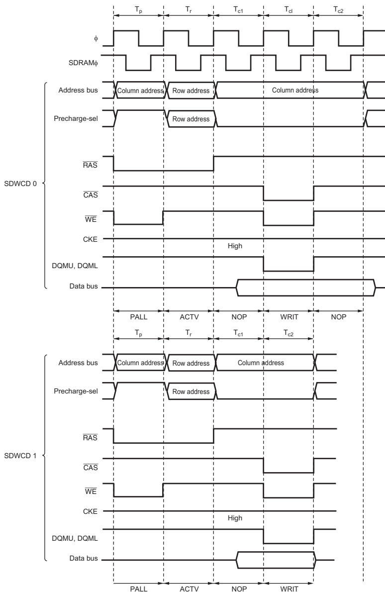
Figure 6.5 CAS Latency Control Cycle Disable Timing during Continuous Synchronous DRAM Space Write Access (for CAS Latency 2)
