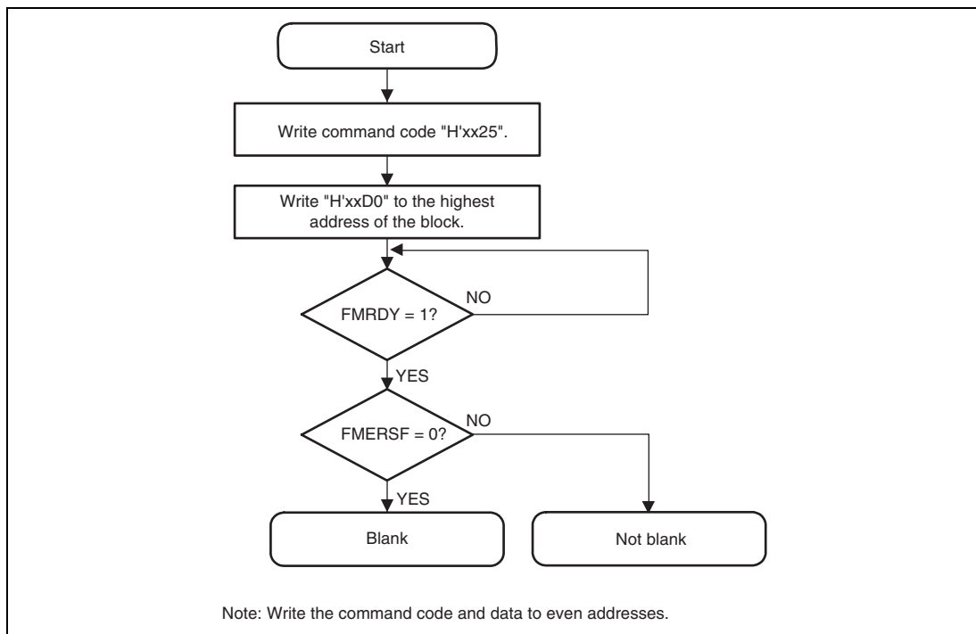
Figure 21.6 Flowchart of Block Blank Check Command Processing
