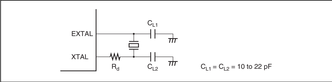
Figure 23.2 Connection of Crystal Resonator (Example)
