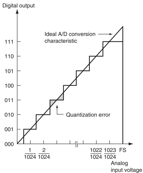
Figure 17.9 A/D Conversion Accuracy Definitions
