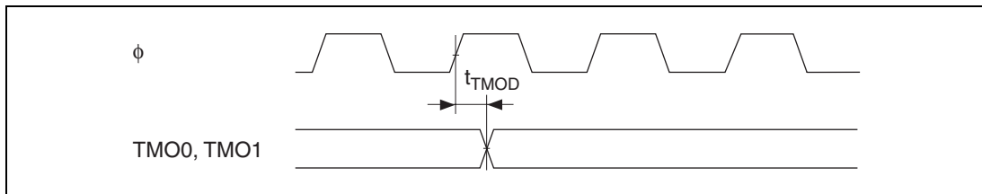
Figure 26.40 8-Bit Timer Output Timing
