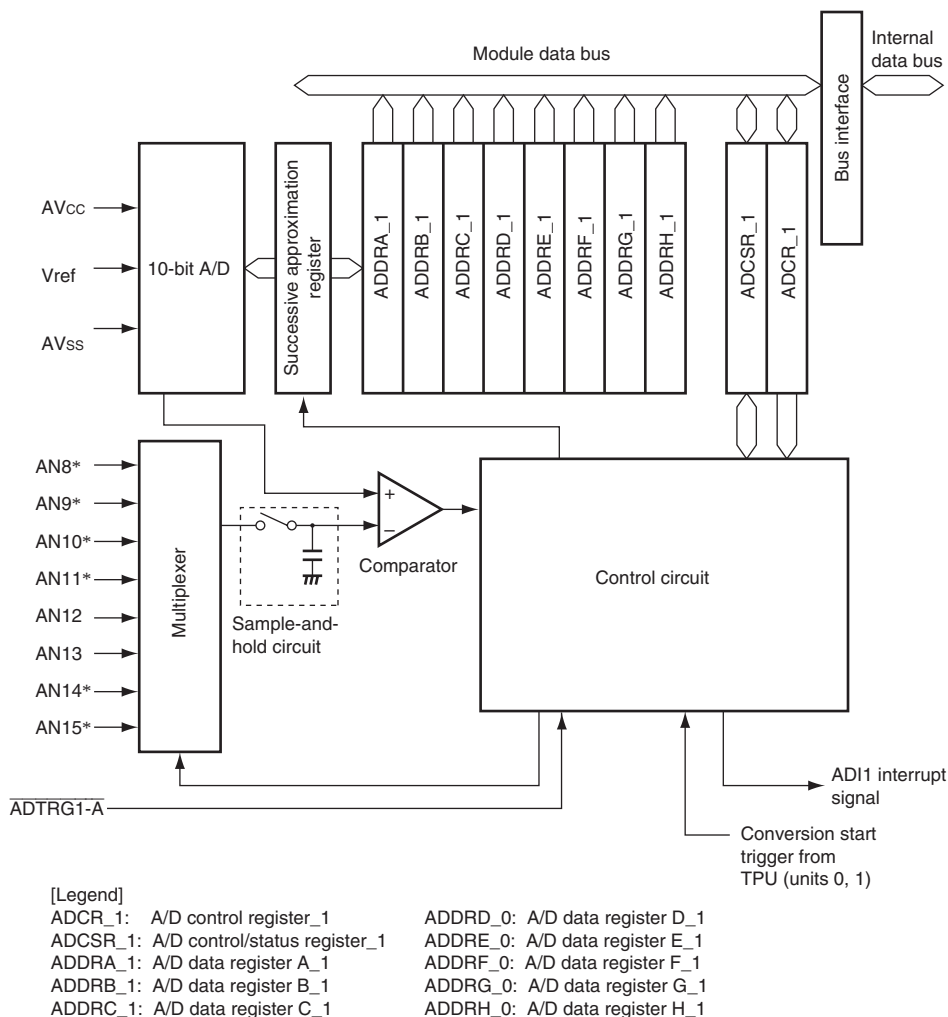
Figure 17.2 Block Diagram of A/D Converter Unit 1 (AD_1)
