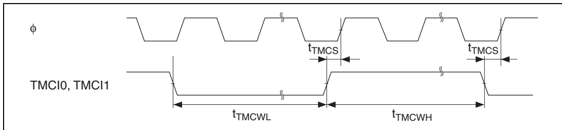
Figure 26.41 8-Bit Timer Clock Input Timing
