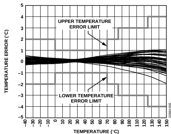
Figure 11. Temperature Accuracy of 40 ADT7301s @ 3.3 V
