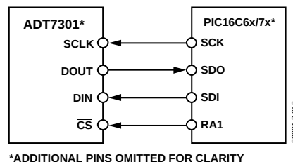
Figure 17. ADT7301-to-PIC16C6x/7x Interface
