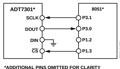
Figure 16. ADT7301-to-8051 Interface
