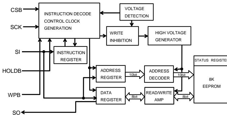
Figure 5. Block diagram
