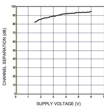
Channel separation vs. supply voltage
