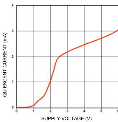
Quiescent current vs. supply voltage
