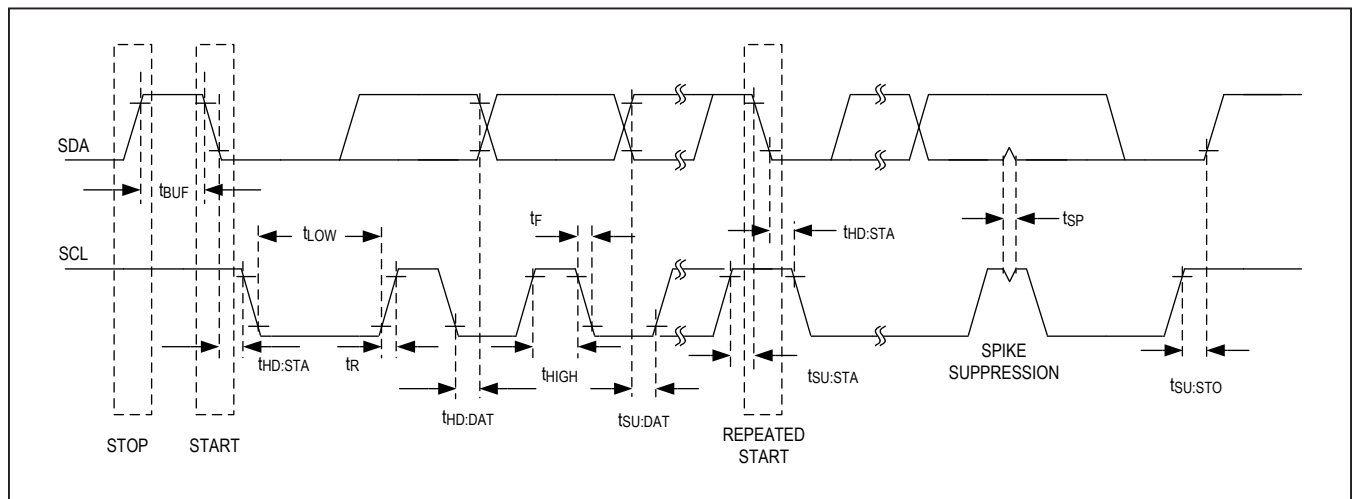
Figure 43: I 2 C Timing Diagram
