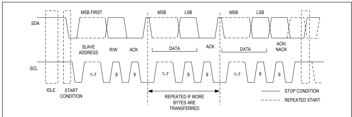
Figure 41. I 2 C Protocol Overview
