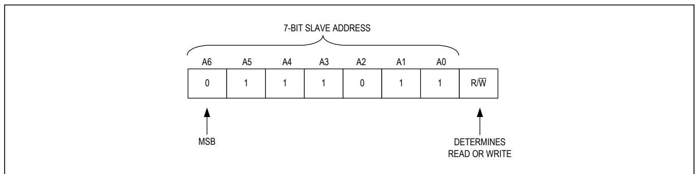
Figure 42. DS2476 I 2 C Slave Address
