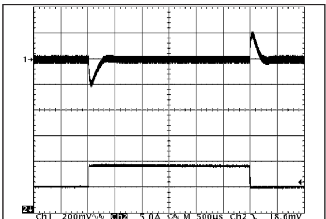
Figure 12: Output voltage response to step-change in load current (50%-75%-50% of I_{out(max)} ; dI/dt = 5A/\mu s ). Load cap: 470μF, 30 mΩ ESR tantalum capacitor and 1μF ceramic cap. Ch 1: V_{out} (200mV/div), Ch 2: I_{out} (5A/div).
