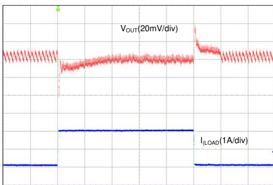
Figure 100. Transient Load Step Response, AUTO Mode (3-Phase Output)
