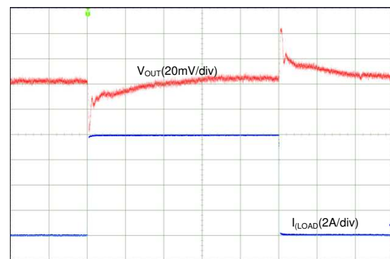
Figure 101. Transient Load Step Response, AUTO Mode (2-Phase Output)
