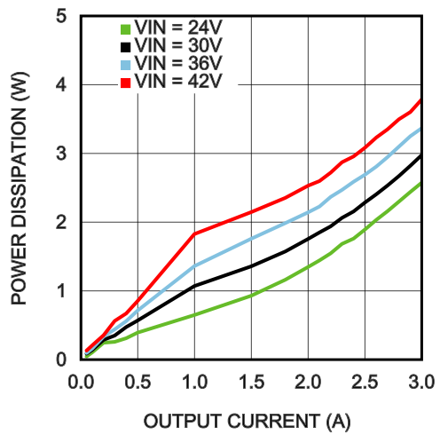
Power Dissipation V_{OUT} = 18V T_{AMB} = 25^{\circ}C
