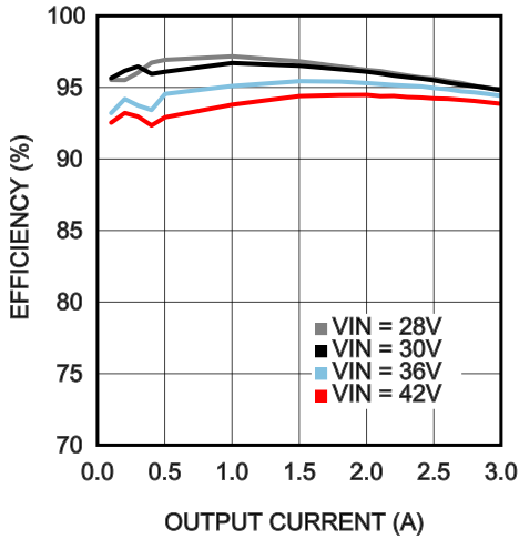
Efficiency V_{OUT} = 24V T_{AMB} = 85^{\circ}C
