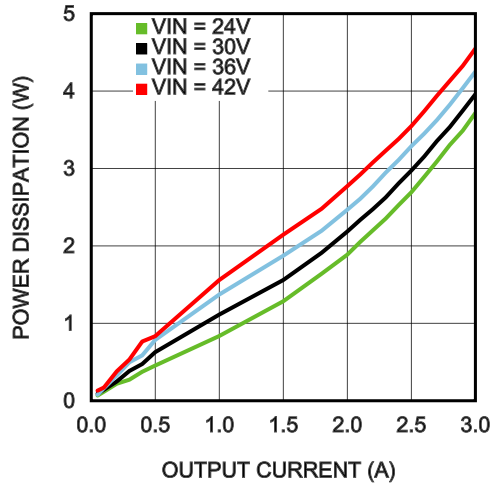
Power Dissipation V_{OUT} = 15V T_{AMB} = 85^{\circ}C
