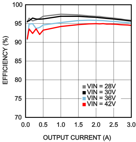
Efficiency V_{OUT} = 24V T_{AMB} = 25^{\circ}C
