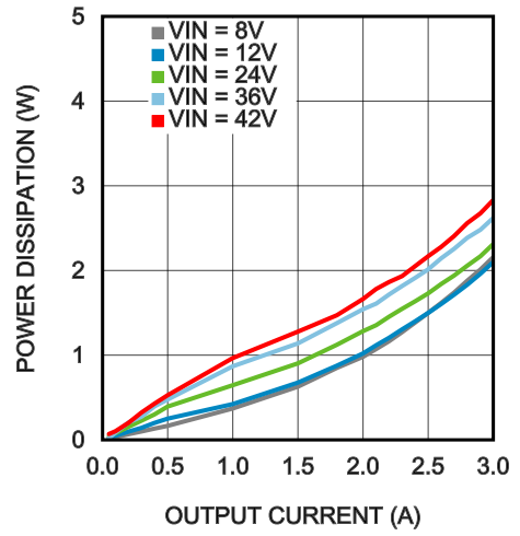
Power Dissipation V_{OUT} = 5.0V T_{AMB} = 25^\circ C
