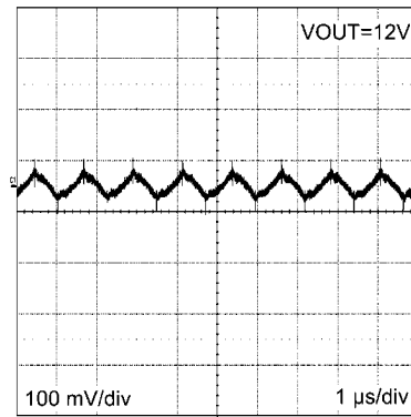
Output Ripple V_{IN} = 24V, I_{OUT} = 3A, \text{Polymer Electrolytic } C_{OUT}, BW = 200 \text{ MHz}
