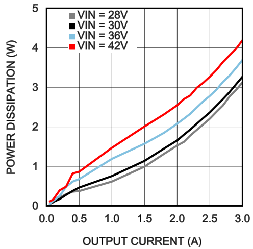
Power Dissipation V_{OUT} = 24V T_{AMB} = 25^{\circ}C
