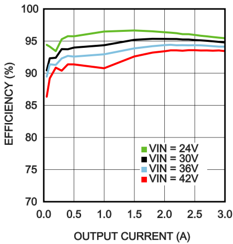
Efficiency V_{OUT} = 18V T_{AMB} = 25^{\circ}C
