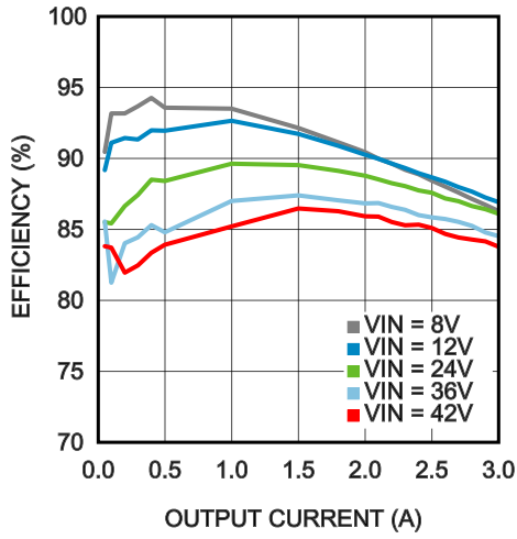
Efficiency V_{OUT} = 5.0V T_{AMB} = 25^\circ C
