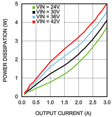
Power Dissipation V_{OUT} = 18V T_{AMB} = 85^{\circ}C
