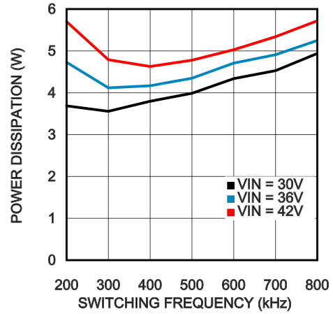
Switching Frequency vs. Power Dissipation V_{OUT} = 24V
