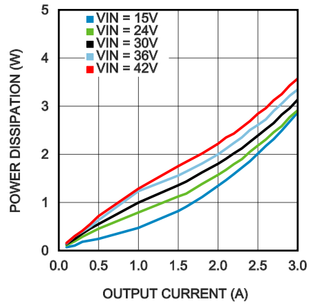
Power Dissipation V_{OUT} = 12V T_{AMB} = 25^\circ C
