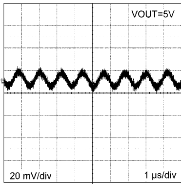
Output Ripple V_{IN} = 12V, I_{OUT} = 3A, \text{Ceramic } C_{OUT}, BW = 200 \text{ MHz}
