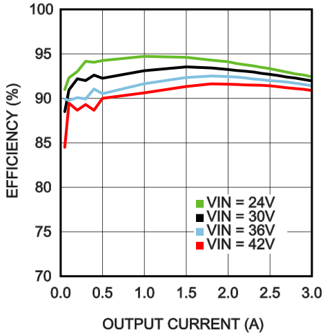
Efficiency V_{OUT} = 15V T_{AMB} = 85^{\circ}C
