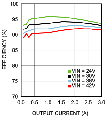
Efficiency V_{OUT} = 18V T_{AMB} = 85^{\circ}C
