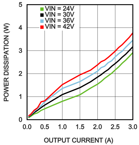
Power Dissipation V_{OUT} = 15V T_{AMB} = 25^{\circ}C
