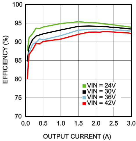
Efficiency V_{OUT} = 15V T_{AMB} = 25^{\circ}C
