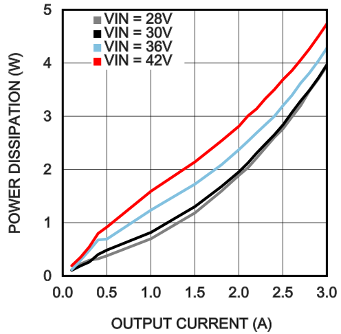
Power Dissipation V_{OUT} = 24V T_{AMB} = 85^{\circ}C
