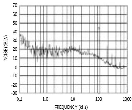
MAX853 NOISE SPECTRUM
