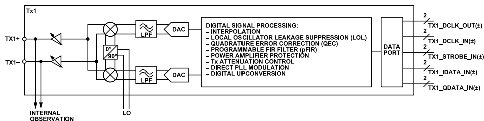
Figure 10. Transmitter Architecture
