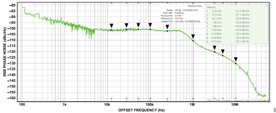
Figure 9. Internal Local Oscillator Phase Noise at 5800 MHz LO
