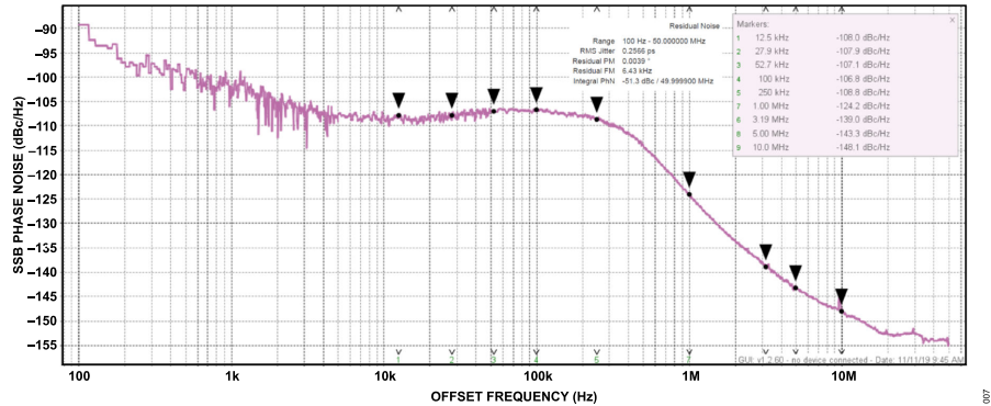
Figure 7. Internal Local Oscillator Phase Noise at 2400 MHz LO
