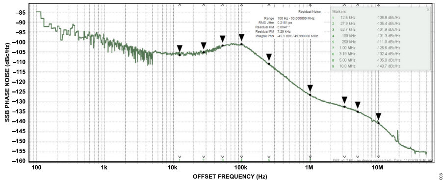
Figure 8. Internal Local Oscillator Phase Noise at 3500 MHz LO
