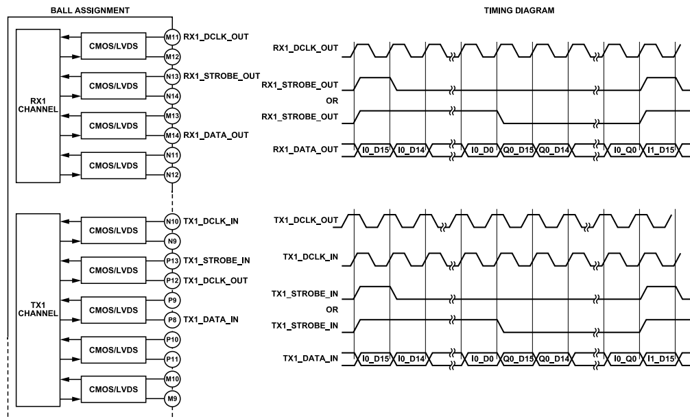
Figure 13. CSSI in 1-Lane Data Mode
