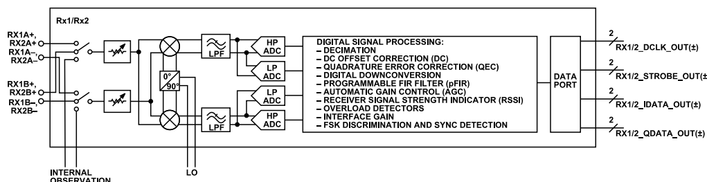
Figure 11. Receiver Architecture
