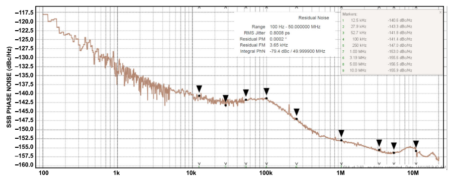
Figure 4. Internal Local Oscillator Phase Noise at 30 MHz LO
