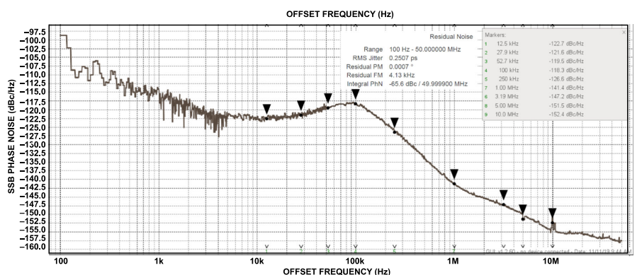
Figure 5. Internal Local Oscillator Phase Noise at 470 MHz LO
