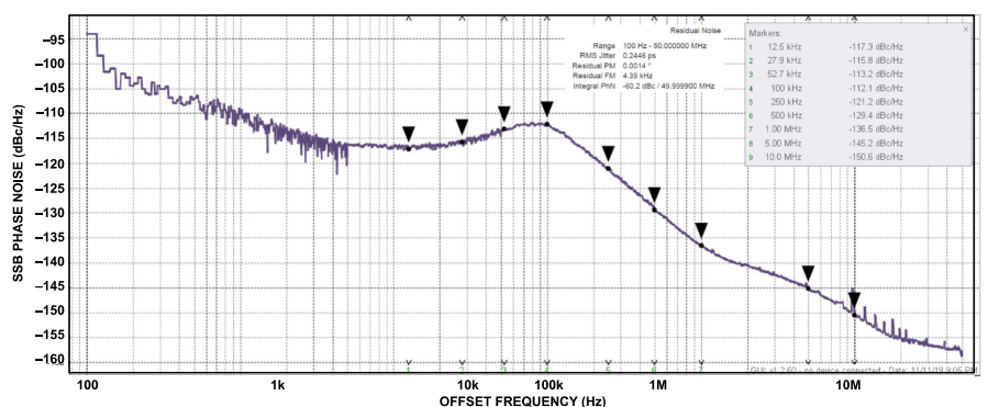
Figure 6. Internal Local Oscillator Phase Noise at 900 MHz LO
