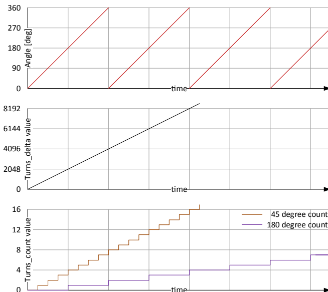
Figure 16: Turn Counting
