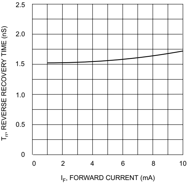
Fig. 1. Reverse Recovery Time vs. Forward Current
