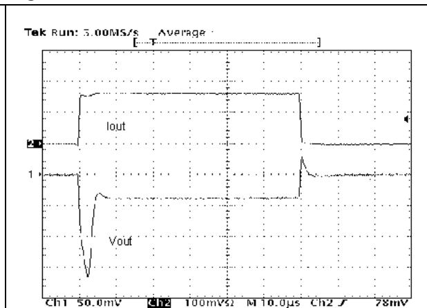
Figure 16. Load transient
