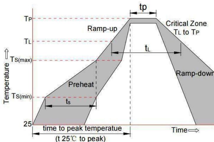
FIG.2: Reflow condition
