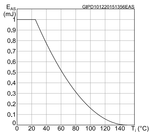
Figure 23: Maximum avalanche energy vs T_J
