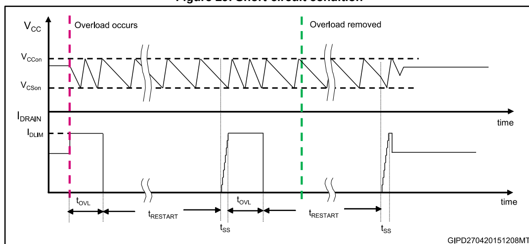
Figure 29: Short-circuit condition
