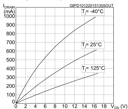
Figure 21: Output characteristic
