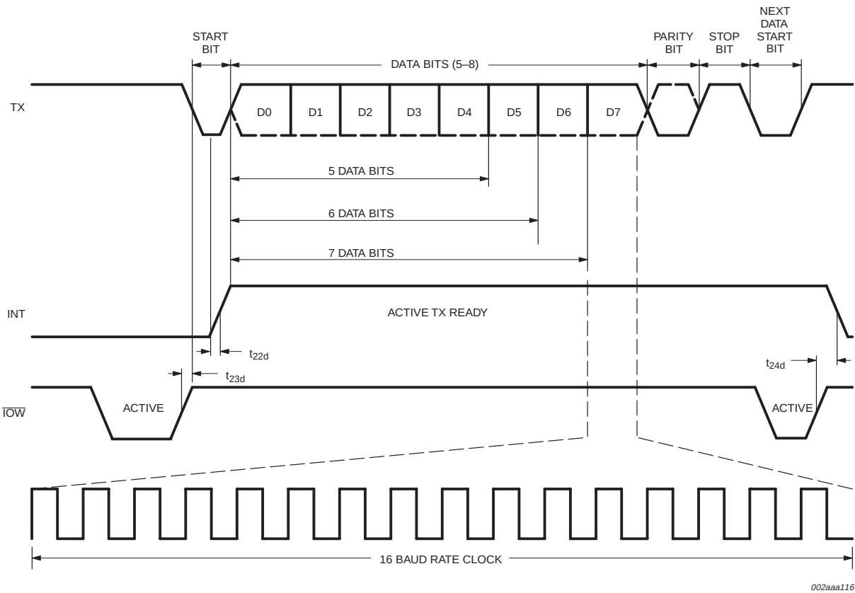
Fig 12. Transmit timing.
