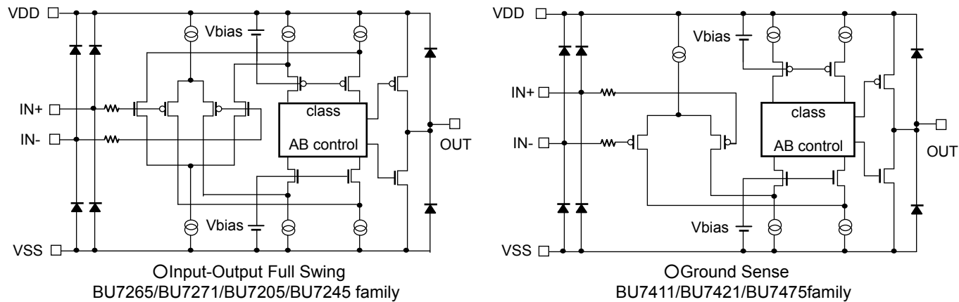
Fig.162 Schematic Diagram
