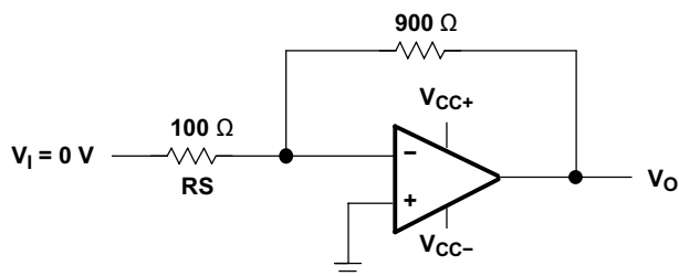
Figure 7-2. Noise-Test Circuit
