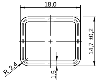
0,5mm Recommended Tin Paste Mask Layer
