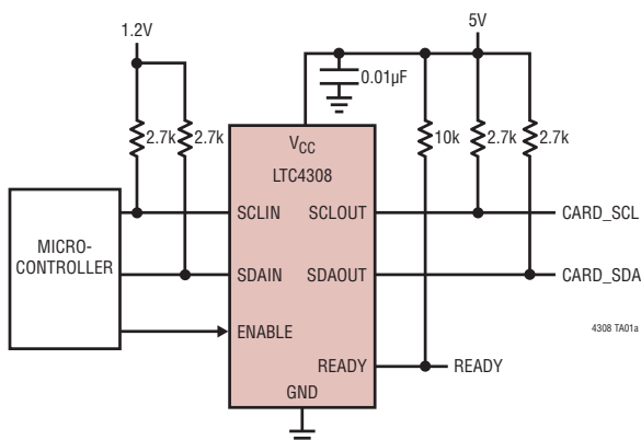
The LTC4308 in a 1.2V Microcontroller Application
