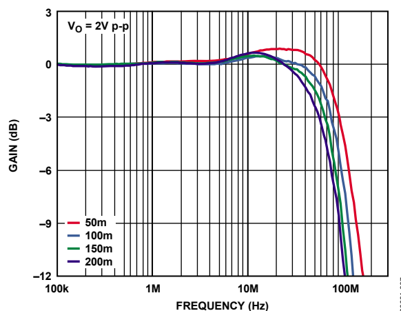
Figure 7. Equalized Frequency Response for Various Cable Lengths
