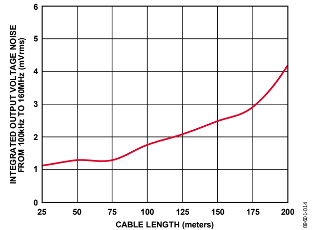
Figure 14. Integrated Output Voltage Noise vs. Cable Lengths
