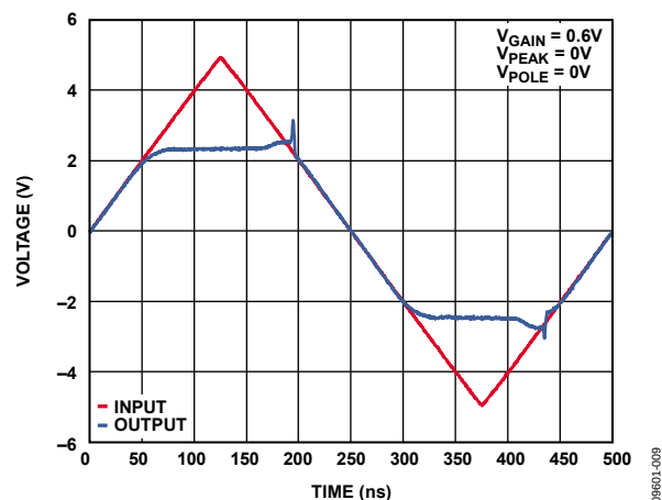
Figure 9. Overdrive Recovery
