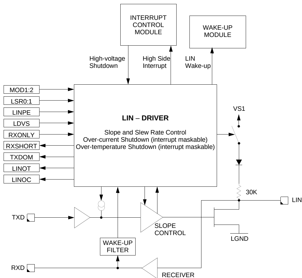
Figure 19. LIN Interface
