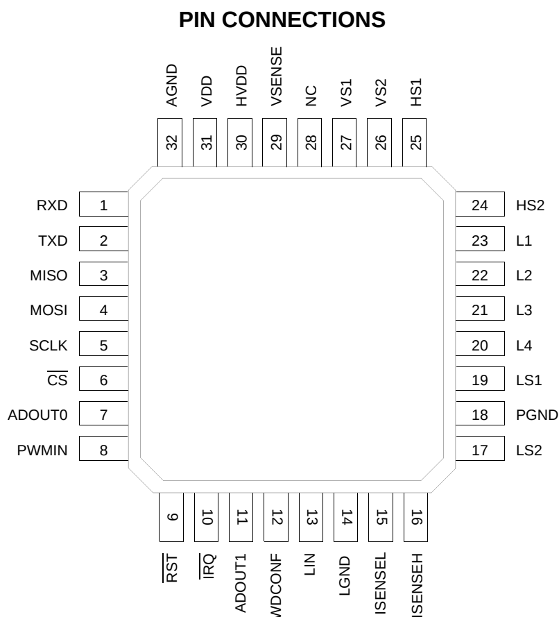
Figure 3. 33912 Pin Connections
