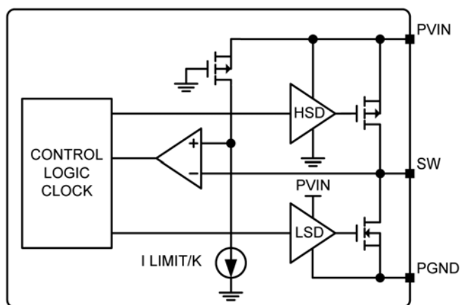
Figure 4. Current-Limit Detail
