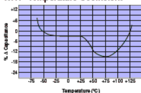
X7R - Temperature Coefficient
