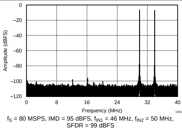
Figure 77. FFT for Two-Tone Input Signal ( -7\text{ dBFS} at 46\text{ MHz} and 50\text{ MHz} )
