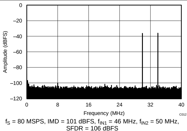
Figure 78. FFT for Two-Tone Input Signal ( -36\text{ dBFS} at 46\text{ MHz} and 50\text{ MHz} )
