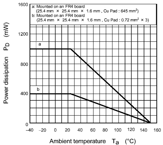
Fig. 7.12 P_D - T_a
