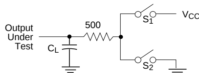
Figure 4. Driver Timing Test Load #2 Circuit
