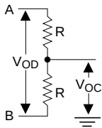
Figure 1. Driver DC Test Load Circuit
