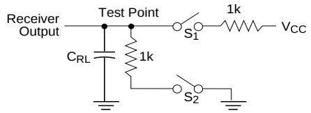
Figure 2. Receiver Timing Test Load Circuit
