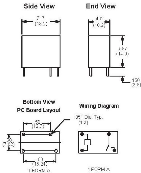
1 FORM A
