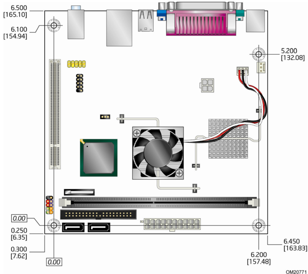
Figure 13. Board Dimensions
