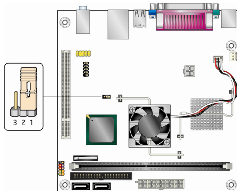
Figure 12. Location of the Jumper Block
