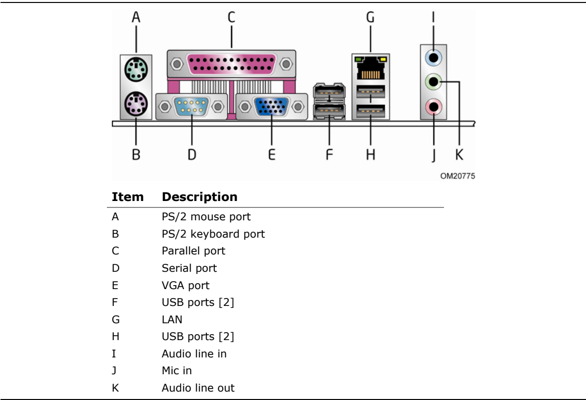
Figure 8. Back Panel Connectors
