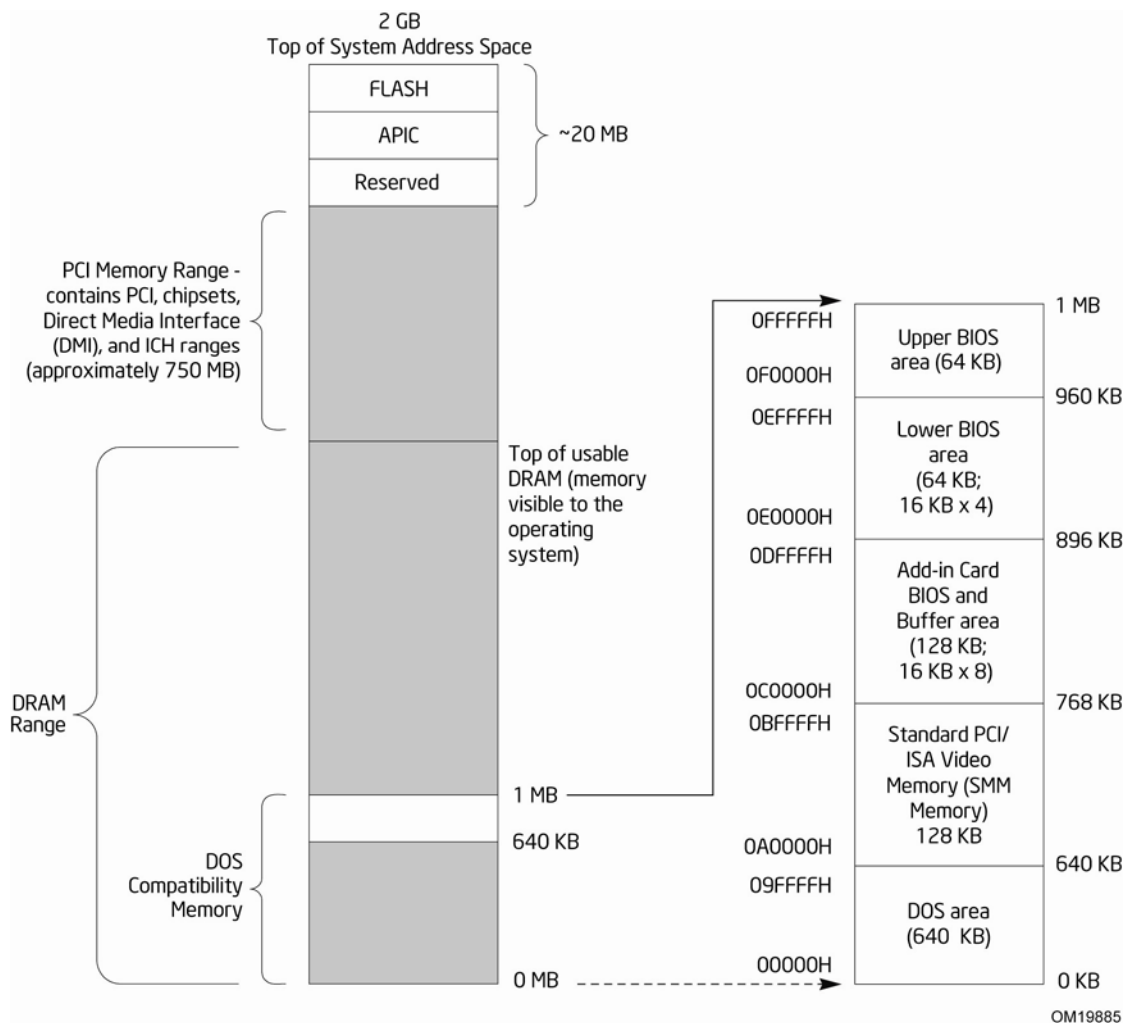
Figure 7. Detailed System Memory Address Map
