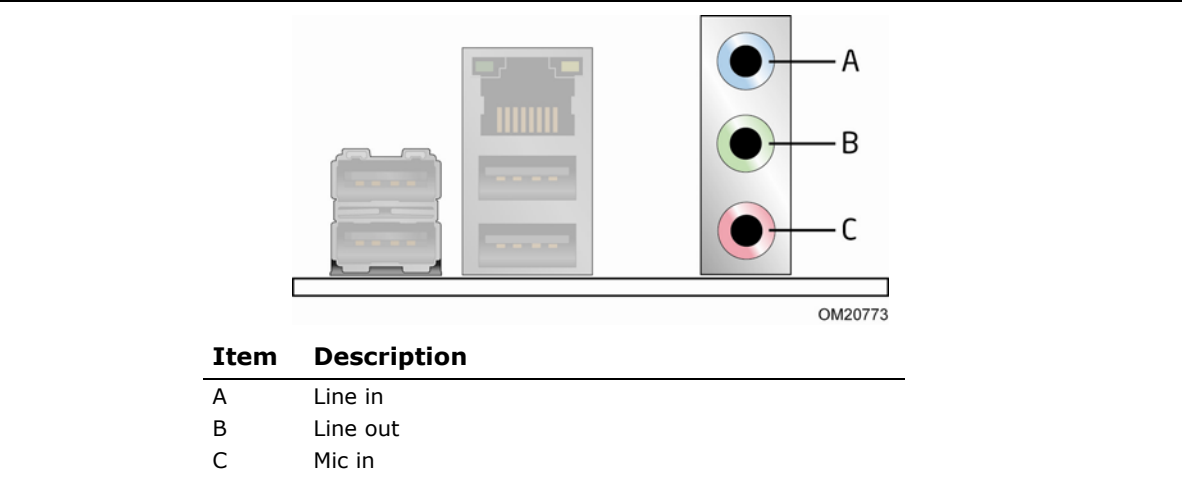
Figure 3. Back Panel Audio Connectors
