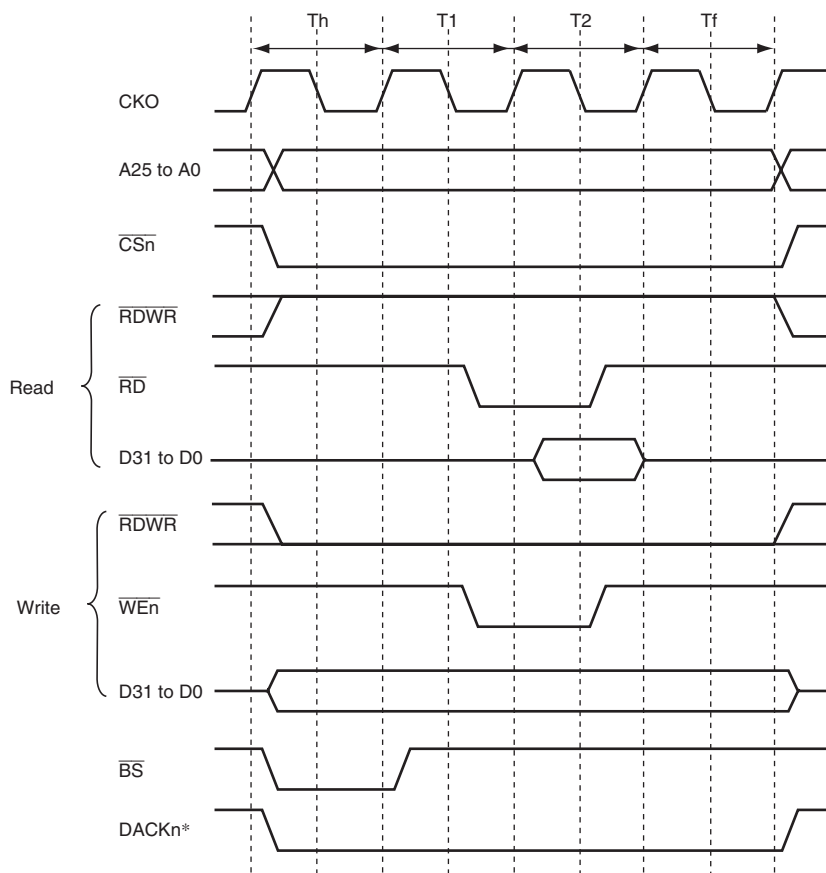
Figure 11.11 \overline{\text{CSn}} Assert Period Expansion
