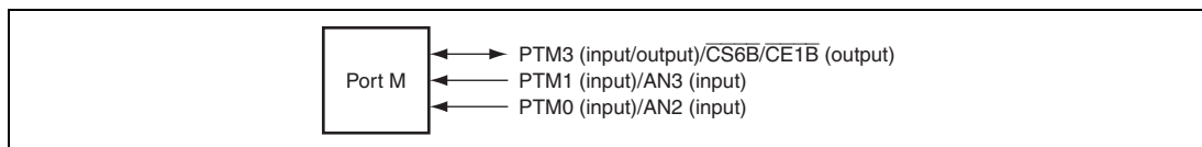
Figure 28.12 Port M
