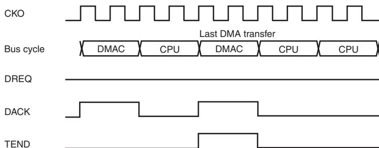
Figure 12.16 DMA Transfer End Signal Timing (Level Detection in Cycle Steal Mode)
