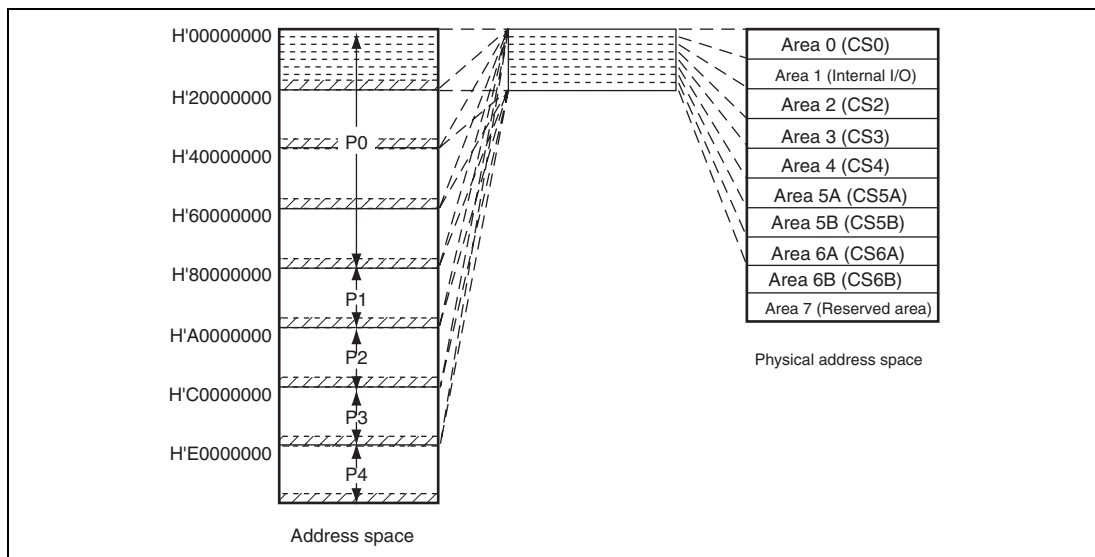
Figure 11.2 Address Space
