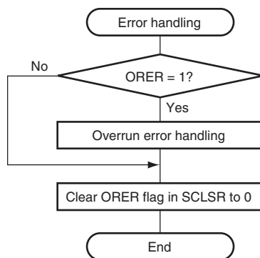
Figure 22.16 Sample Flowchart for Receiving Serial Data (2)
