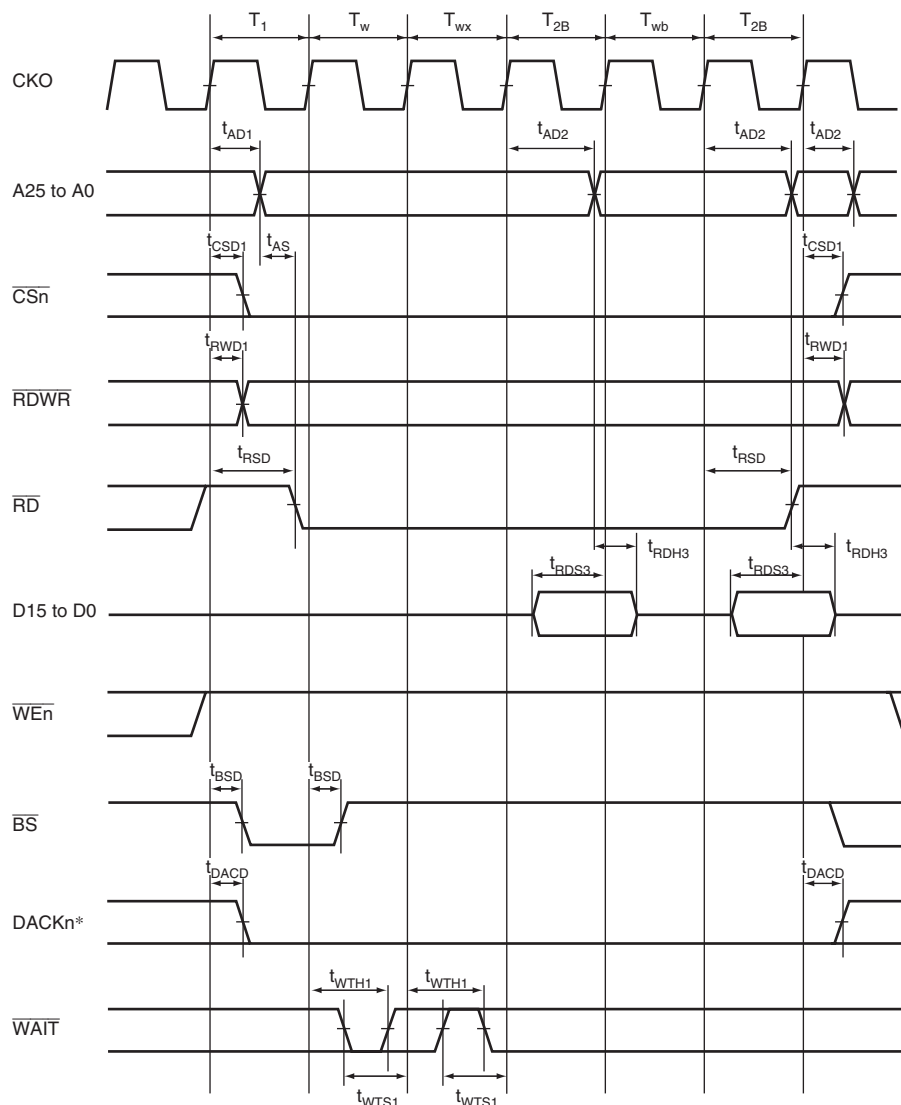
Figure 33.15 Read Bus Cycle of Burst ROM (Software Wait 1, Asynchronous External Wait 1 Input, Burst Wait 1, Number of Burst = 2)
