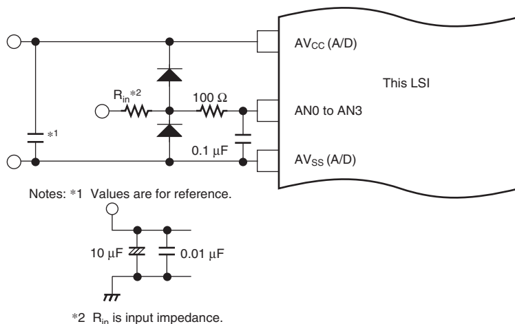
Figure 26.9 Example of Analog Input Protection Circuit
