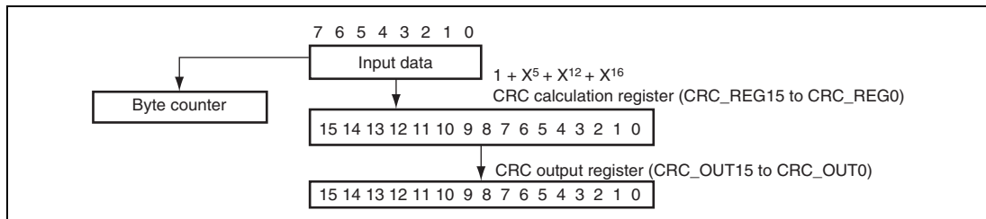
Figure 24.8 CRC Engine Operation
