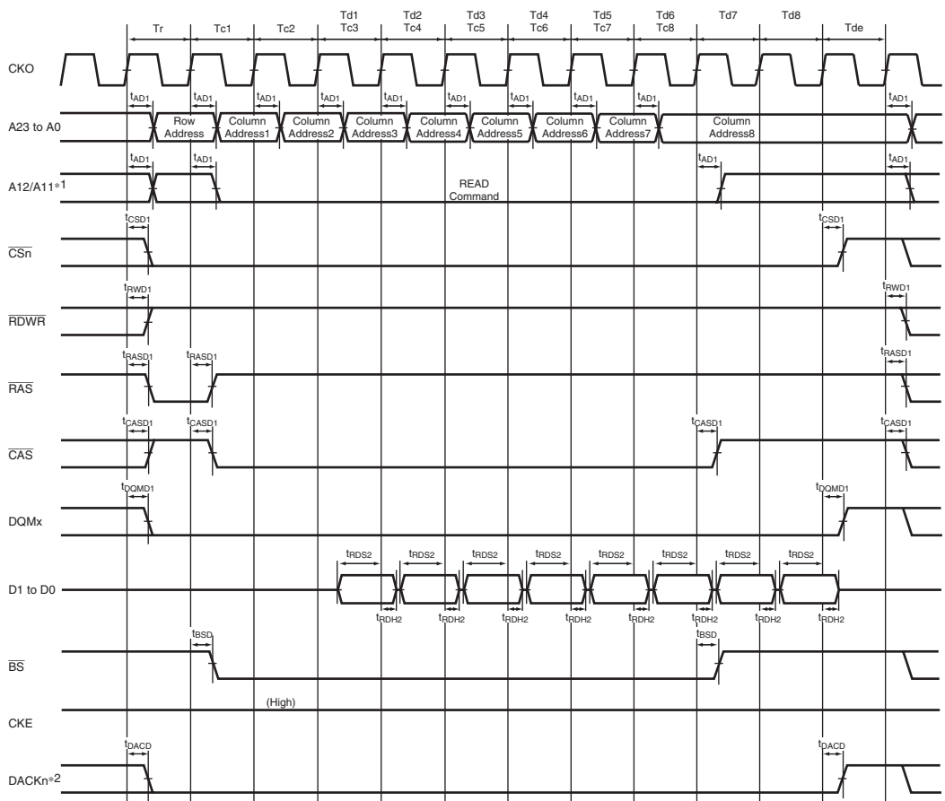
Figure 33.24 Burst Read Bus Cycle of SDRAM (Single Read × 8) (Bank Active Mode: ACTV + READ Command, CAS Latency 2, TRCD = 1 Cycle)
