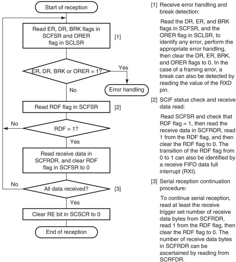
Figure 22.7 Sample Flowchart for Receiving Serial Data
