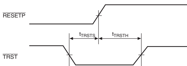
Figure 33.56 \overline{\text{TRST}} Input Timing (Reset Hold)
