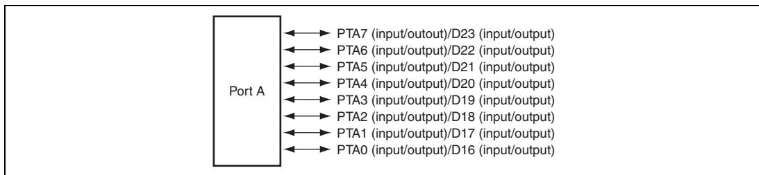
Figure 28.1 Port A
