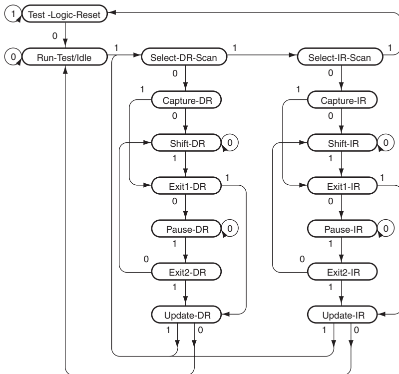
Figure 31.2 TAP Controller State Transitions
