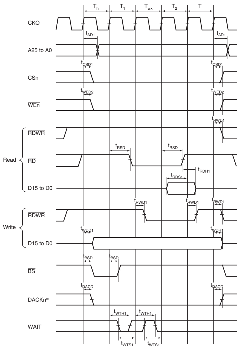
Figure 33.14 Bus Cycle of SRAM with Byte Selection (CSnWCR.SW[1:0]=B'01, CSnWCR.HW[1:0]=B'01, External Wait 1 Input, BAS = 1 (WE in Write Cycle Controlled))
