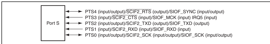
Figure 28.16 Port S
