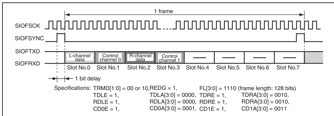
Figure 21.19 Transmit and Receive Timing (16-Bit Stereo Data (4))
