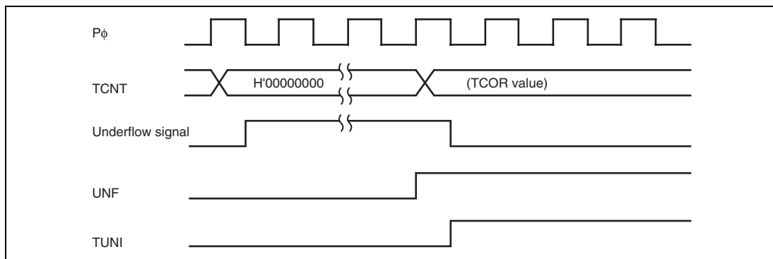
Figure 18.5 UNF Set Timing
