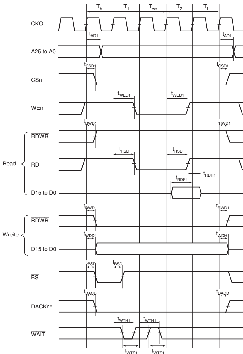
Figure 33.13 Bus Cycle of SRAM with Byte Selection ( \overline{CS_nWCR.SW}[1:0]=B'01 , \overline{CS_nWCR.HW}[1:0]=B'01 , External Wait 1 Input, BAS = 0 (UB and LB in Write Cycle Controlled))
