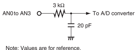
Figure 26.10 Analog Input Pin Equivalent Circuit
