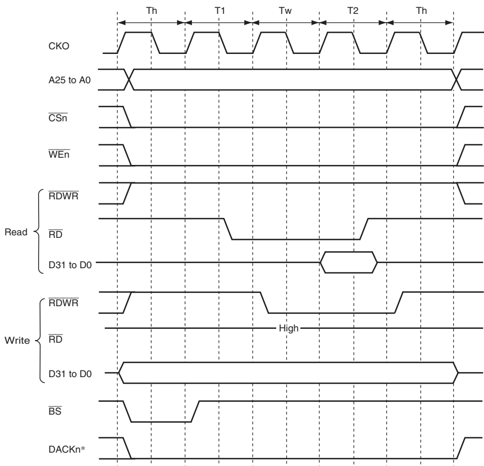
Figure 11.34 Wait Timing for Byte-Selection SRAM (BAS = 1) (Software Wait Only)
