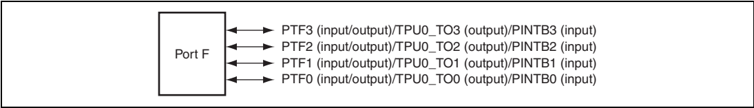
Figure 28.6 Port F
