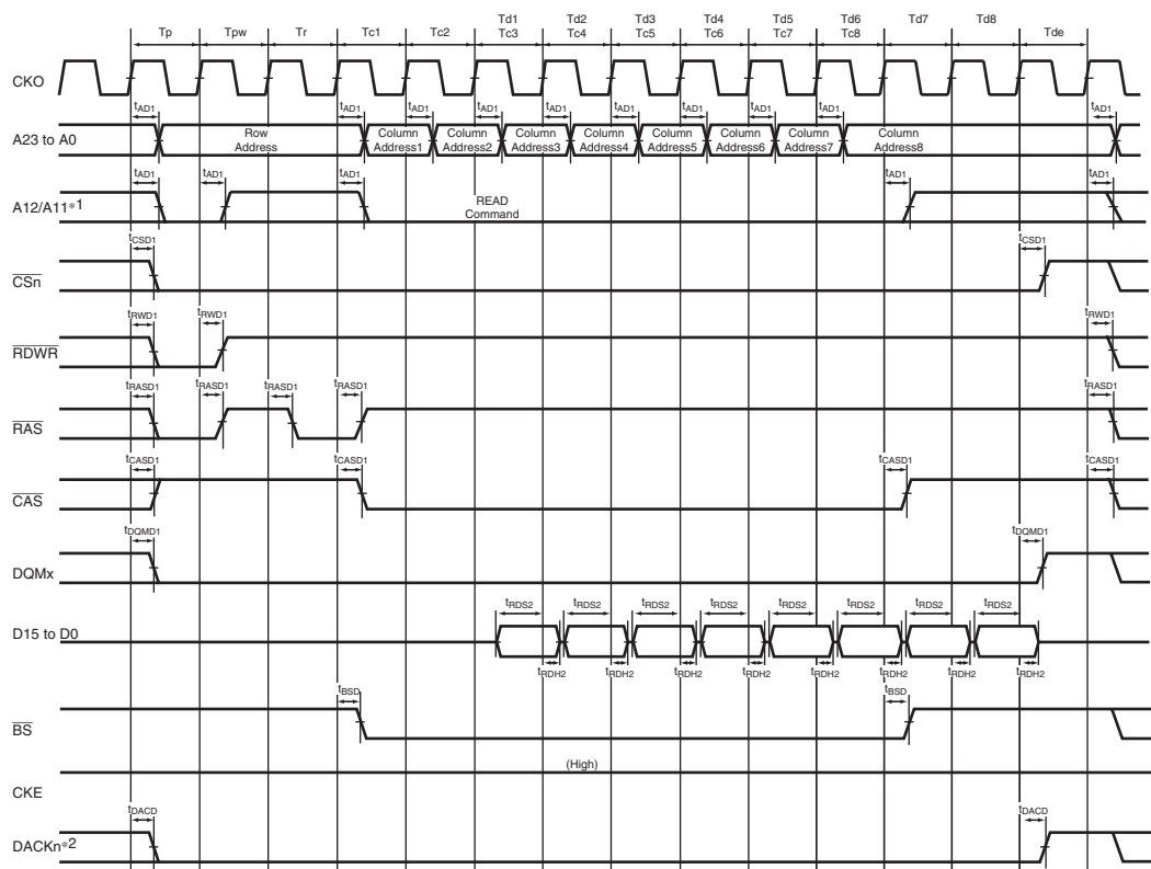
Figure 33.26 Burst Read Bus Cycle of SDRAM (Single Read × 8) (Bank Active Mode: PRE + ACTV + READ Command, Different Row Address, CAS Latency 2, TRCD = 1 Cycle)
