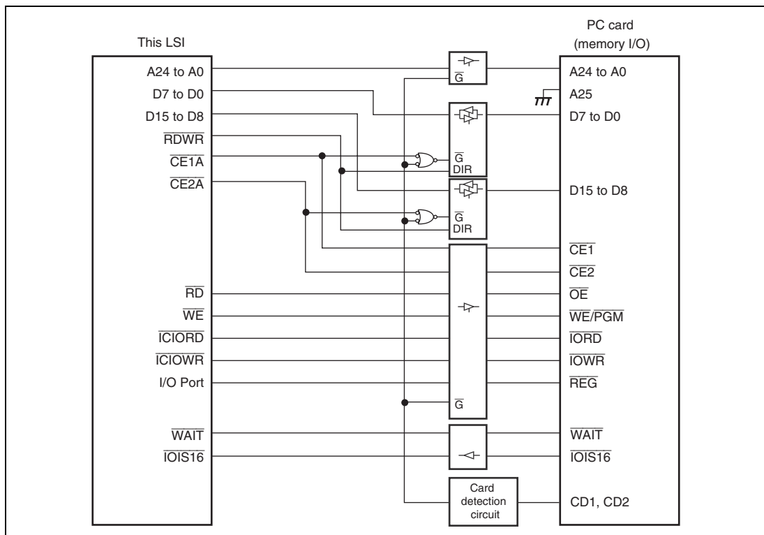
Figure 11.37 Example of PCMCIA Interface Connection
