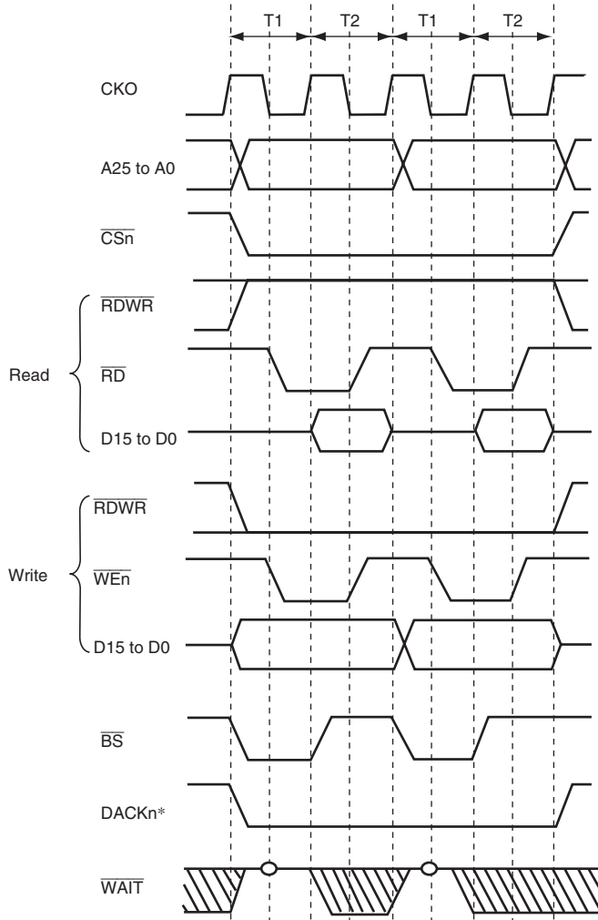
Figure 11.5 Continuous Access for Normal Space 2, Bus Width = 16 bits, Longword Access, CSnWCR.WM Bit = 1 (Access Wait = 0, Cycle Wait = 0)
