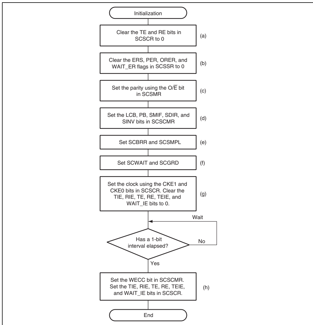
Figure 25.4 Example of Initialization Flow
