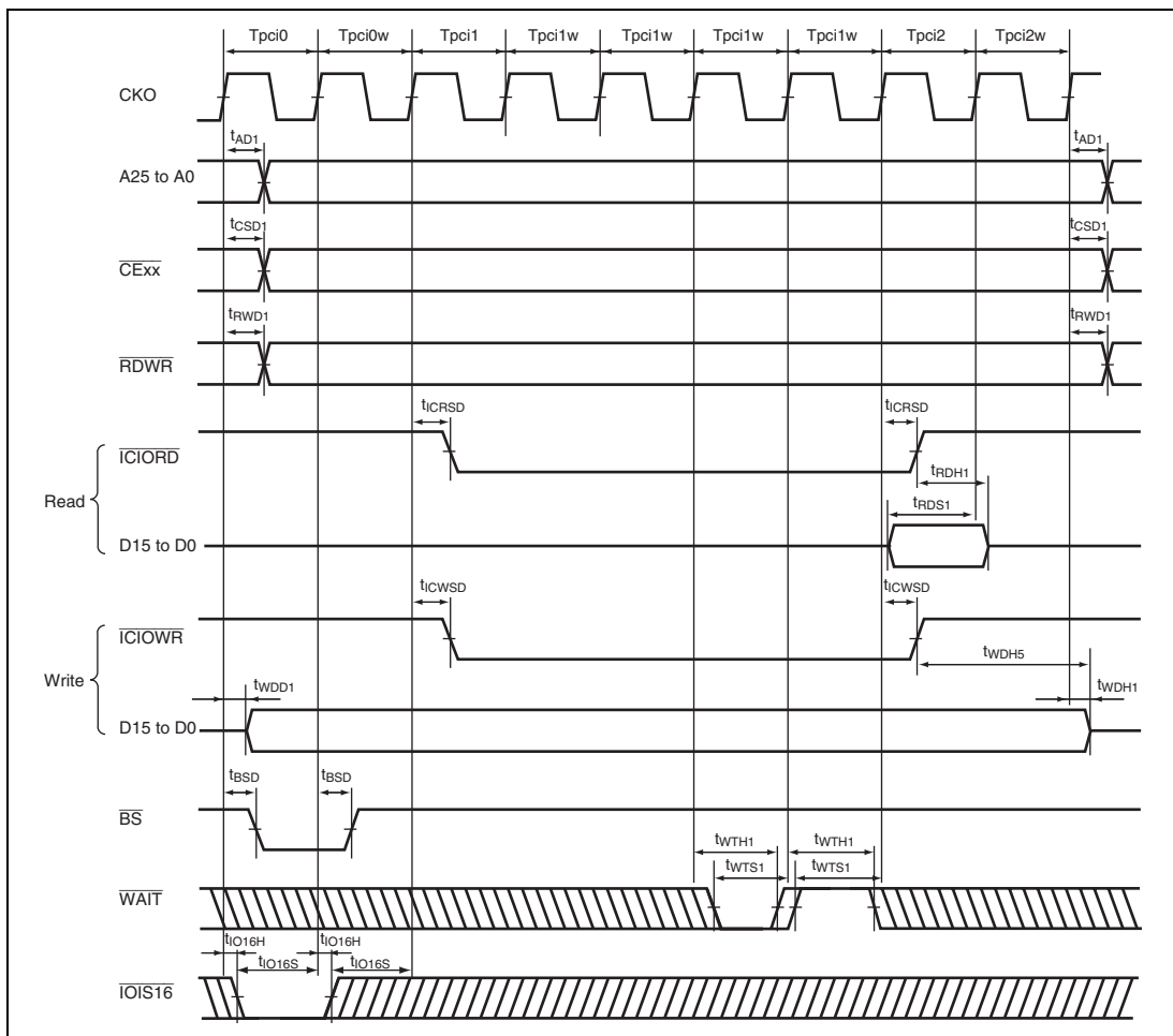
Figure 33.38 PCMCIA I/O Card Interface Bus Timing (TED[3:0] = B'0010, TEH[3:0] = B'0001, Software Wait 1, Hardware Wait 1)
