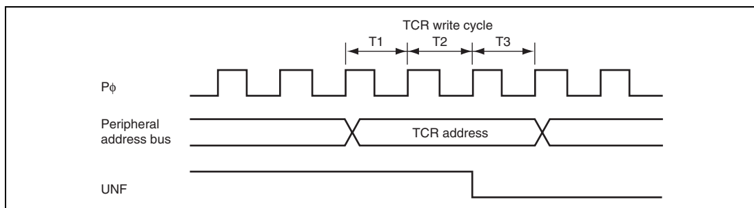
Figure 18.6 Status Flag Clear Timing
