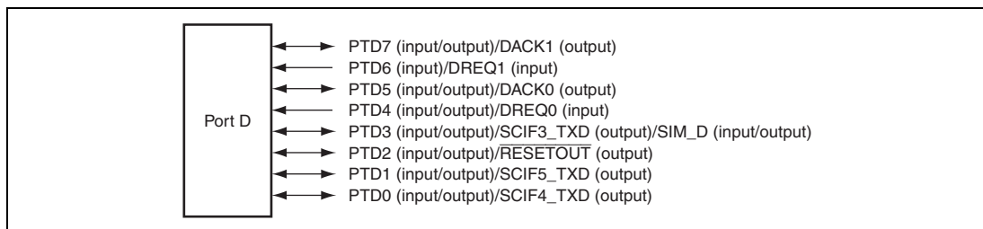
Figure 28.4 Port D
