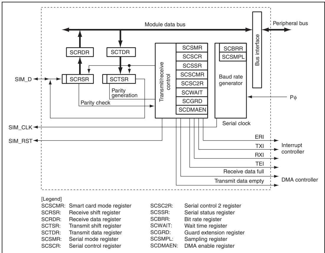
Figure 25.1 Smart Card Interface
