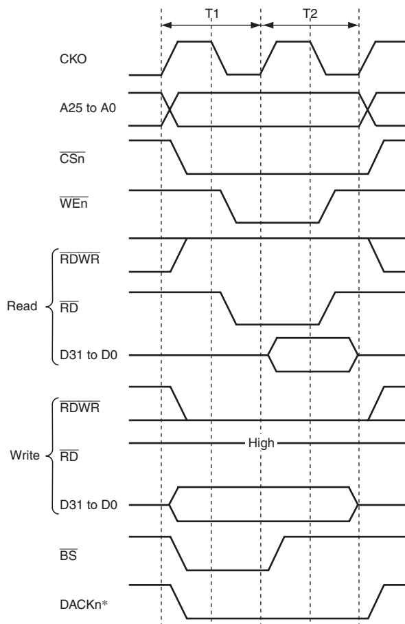
Figure 11.32 Basic Access Timing for Byte-Selection SRAM (BAS = 0)
