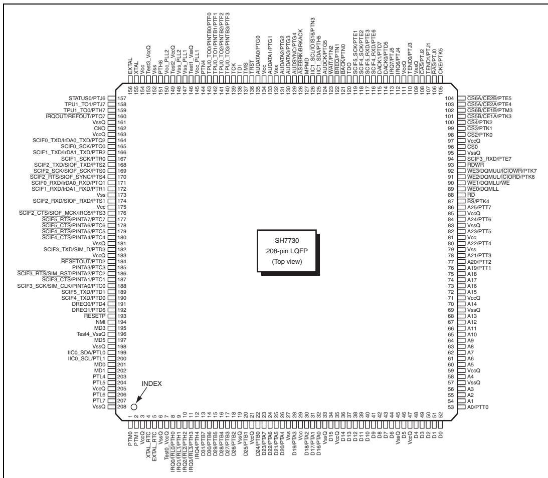
Figure 1.2 Pin Assignments (208-Pin LQFP)
