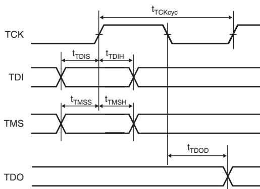
Figure 33.57 H-UDI Data Transfer Timing
