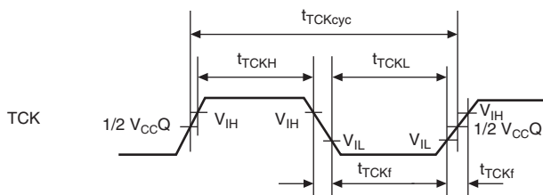
Figure 33.55 TCK Input Timing
