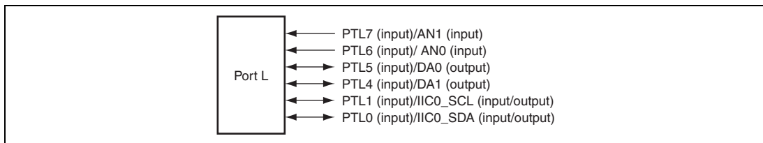
Figure 28.11 Port L
