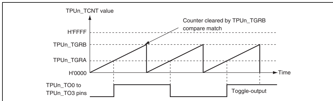
Figure 16.7 Example of Toggle Output Operation
