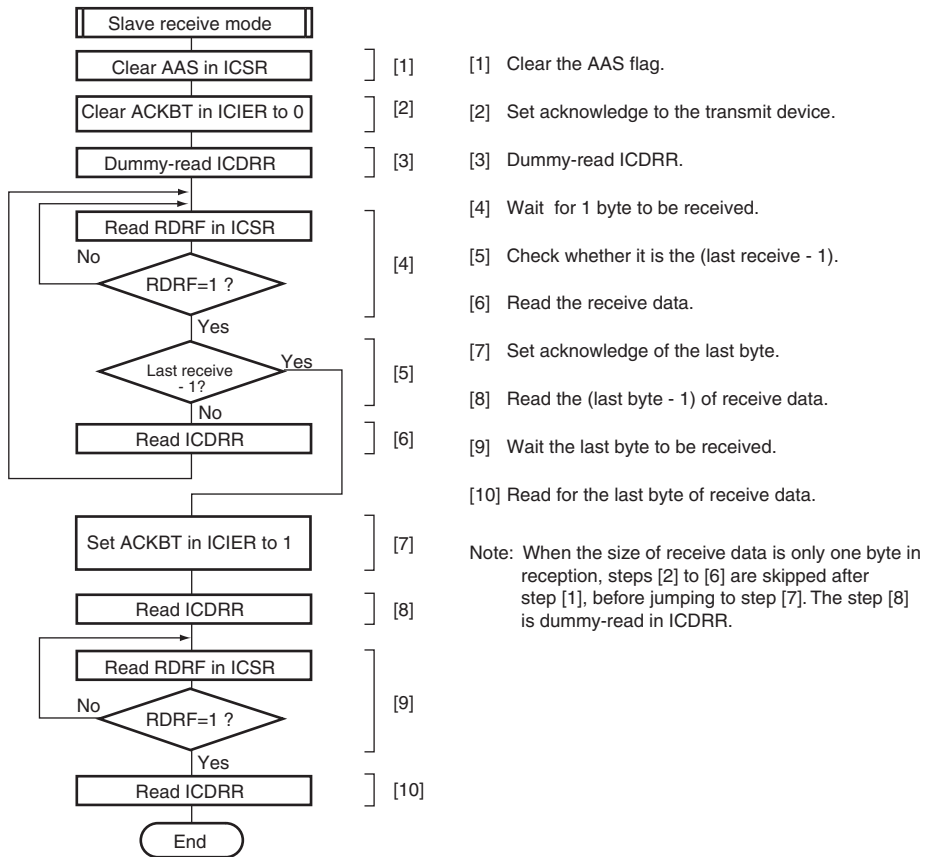
Figure 20.17 Sample Flowchart for Slave Receive Mode
