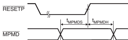
Figure 33.58 \overline{\text{MPMD}} Input Timing
