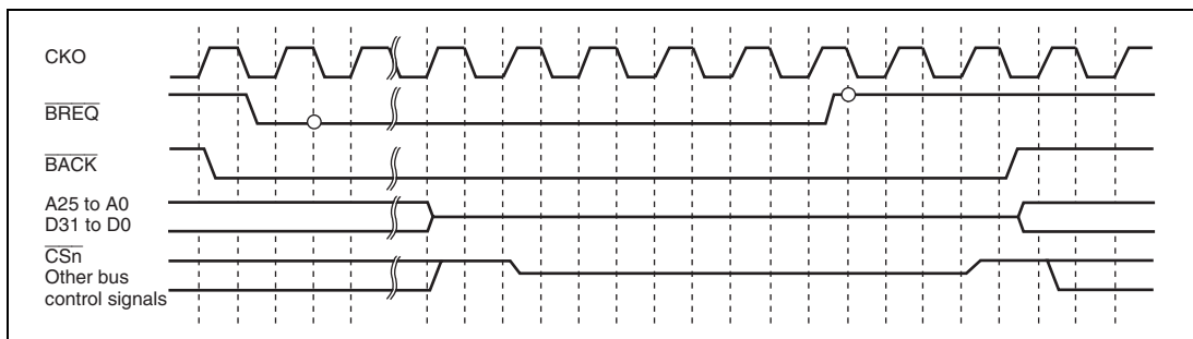
Figure 11.44 Bus Arbitration Timing
