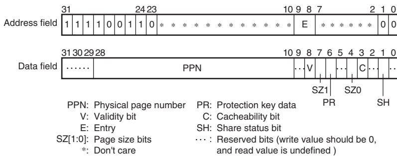
Figure 7.19 Memory-Mapped ITLB Data Array (TLB Compatible Mode)
