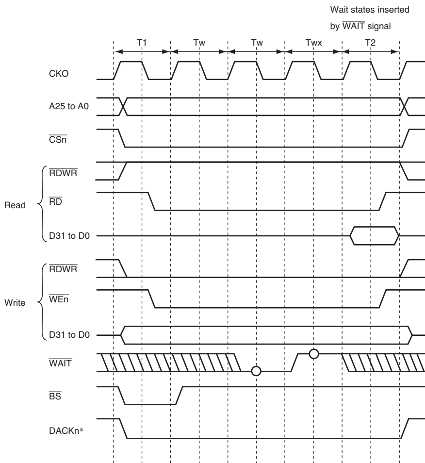
Figure 11.10 Wait State Timing for Normal Space Access (Wait State Insertion using \overline{\text{WAIT}} Signal)
