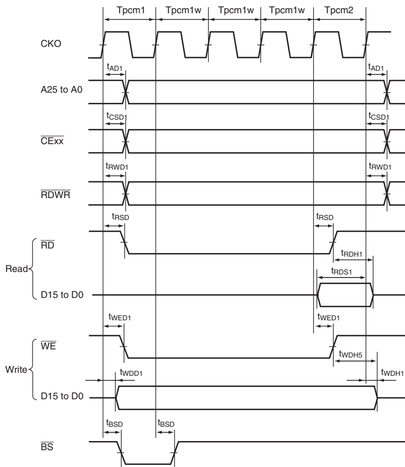
Figure 33.35 PCMCIA Memory Card Interface Bus Timing
