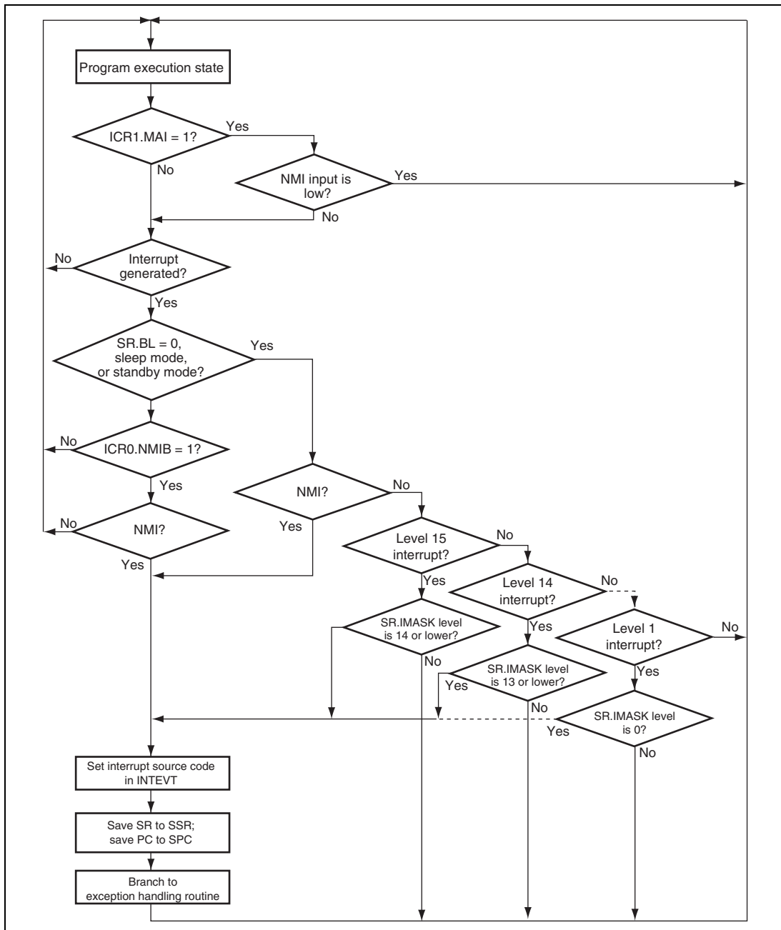
Figure 10.3 Interrupt Operation Flowchart (when CPUOPM.INTMU = 0)
