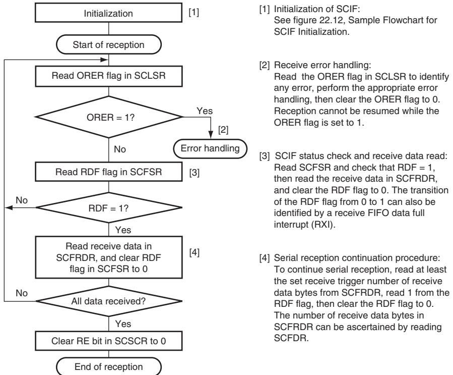
Figure 22.15 Sample Flowchart for Receiving Serial Data (1)
