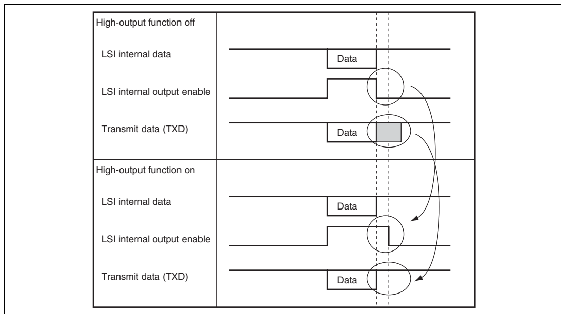
Figure 25.10 High-Output Function Timechart
