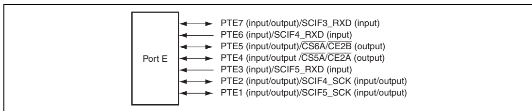
Figure 28.5 Port E
