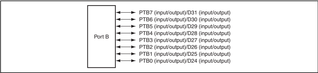
Figure 28.2 Port B
