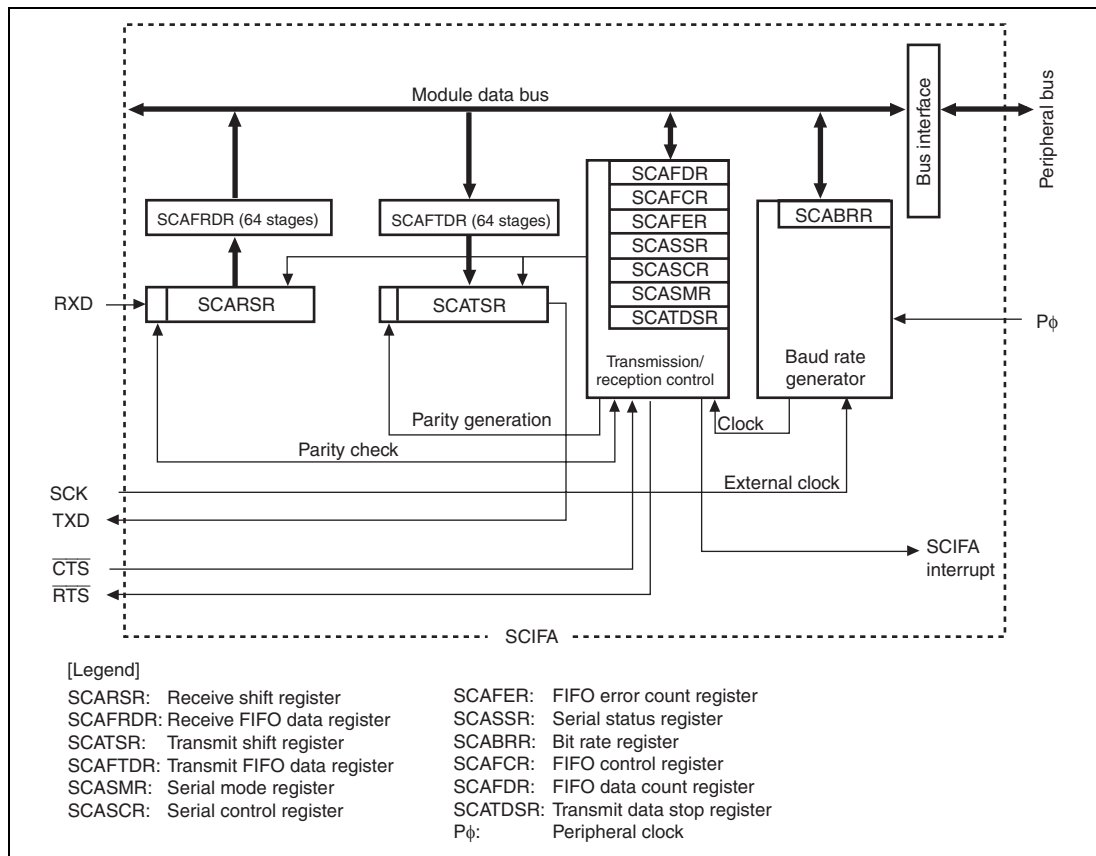
Figure 23.1 Block Diagram of SCIFA
