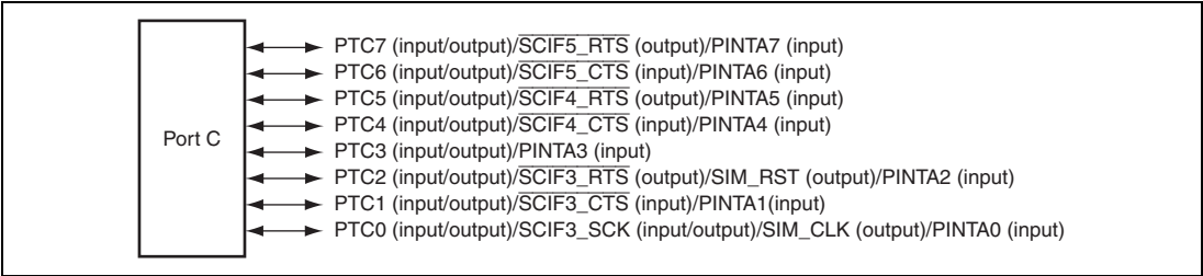
Figure 28.3 Port C
