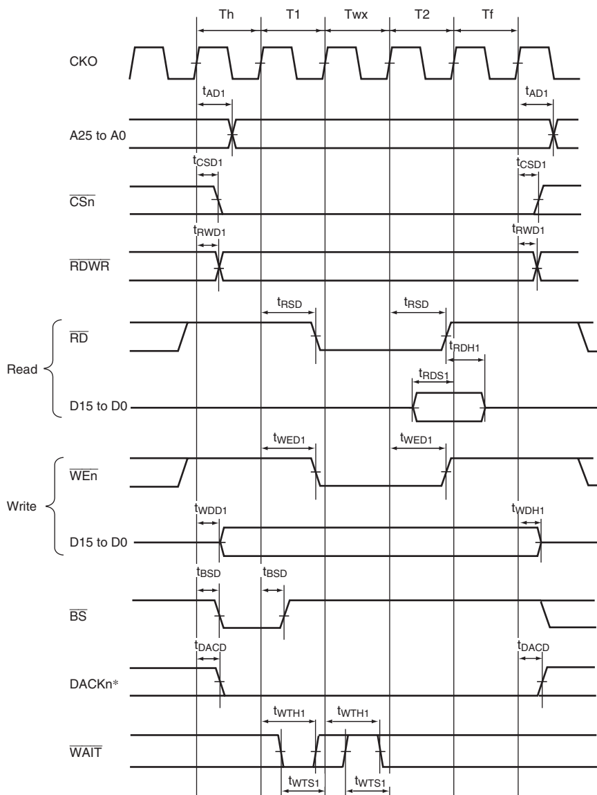
Figure 33.12 CS Extended Bus Cycle in Normal Space ( \overline{CS}_n\overline{WCR.SW}[1:0]=B'01 , \overline{CS}_n\overline{WCR.HW}[1:0]=B'01 , External Wait 1 Input)
