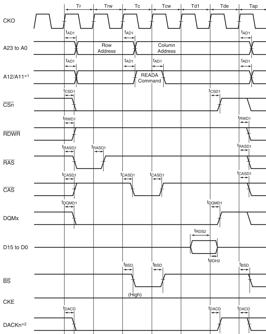
Figure 33.17 Single Read Bus Cycle of SDRAM (Auto Precharge Mode, CAS Latency 2, TRCD = 2 Cycles, TRP = 2 Cycles)
