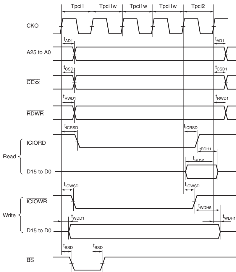
Figure 33.37 PCMCIA I/O Card Interface Bus Timing
