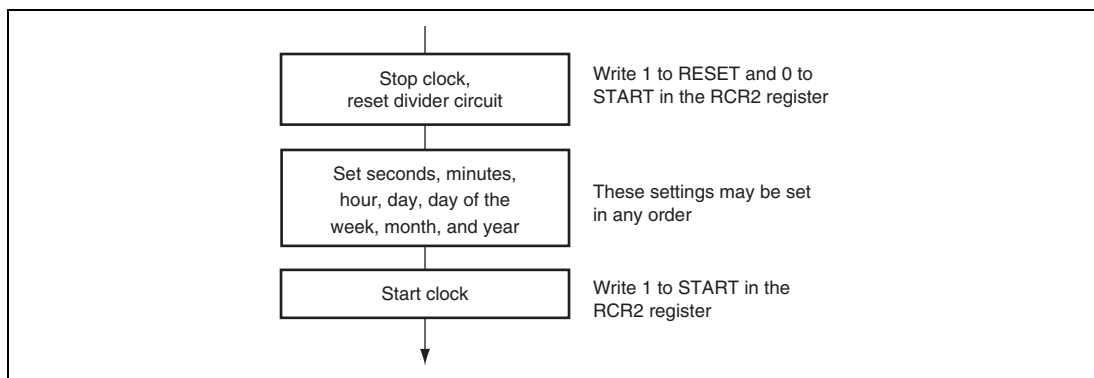
Figure 17.2 Setting Time
