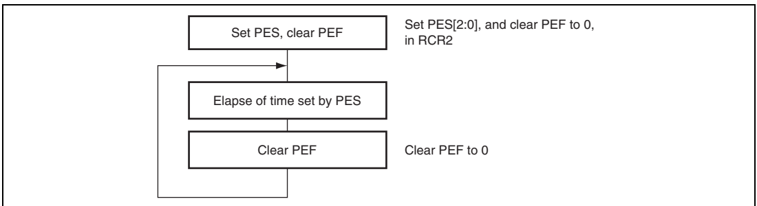
Figure 17.5 Using Periodic Interrupt Function
