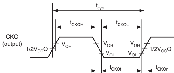
Figure 33.2 CKIO Clock Output Timing
