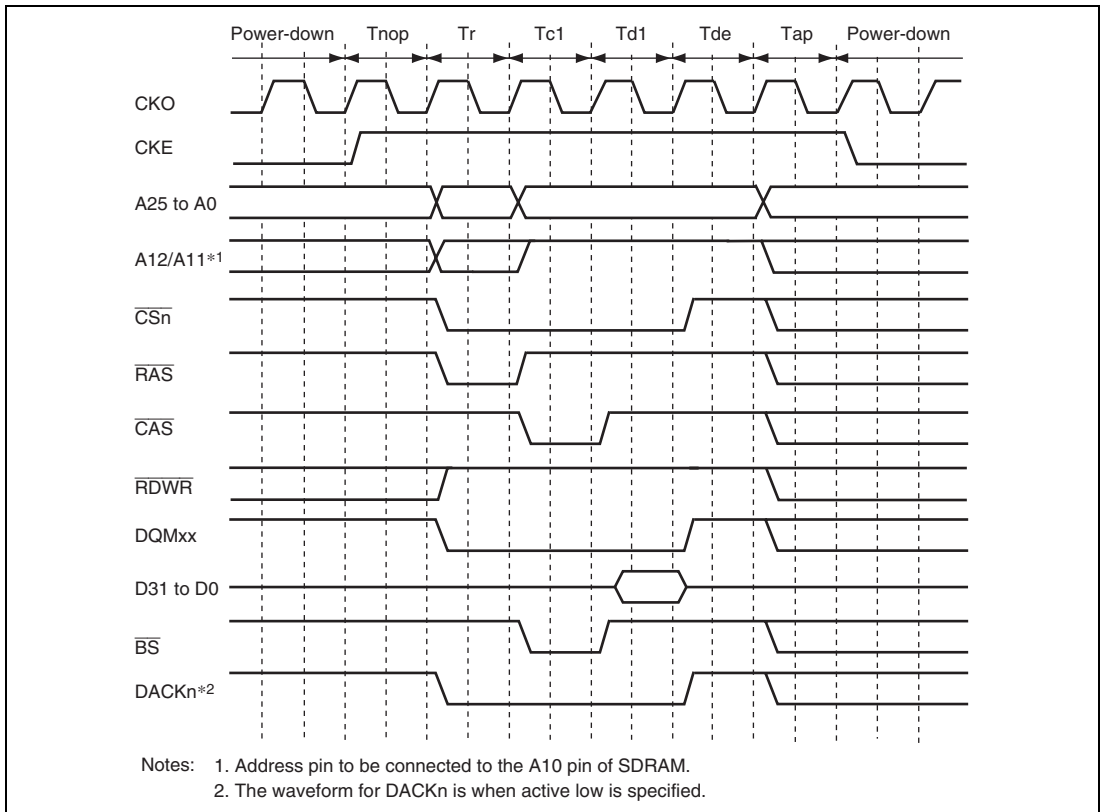
Figure 11.27 Access Timing in Power-Down Mode
