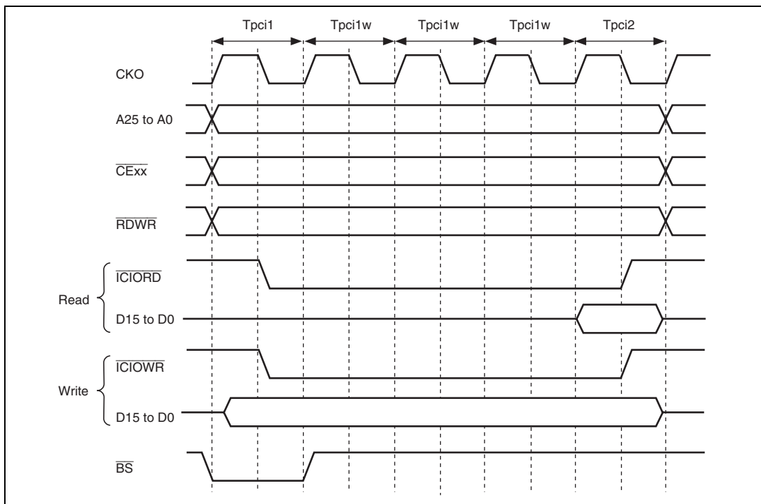
Figure 11.41 Basic Timing for PCMCIA I/O Card Interface
