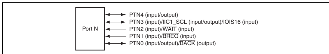
Figure 28.13 Port N
