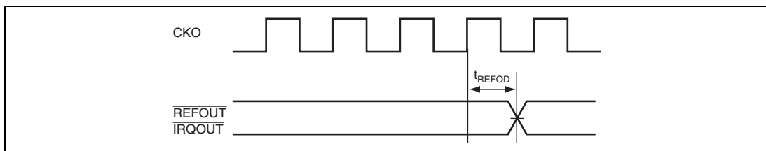
Figure 33.39 \overline{\text{REFOUT}} , \overline{\text{IRQOUT}} Delay Time
