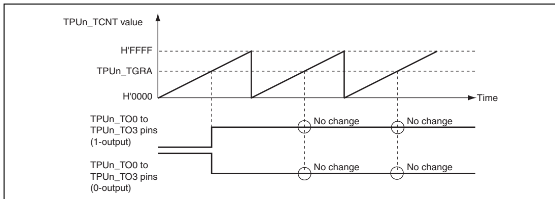
Figure 16.6 Example of 0-Output/1-Output Operation
