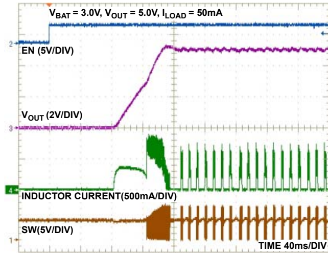
FIGURE 12. START-UP AFTER ENABLE ( I_{LOAD} = 50mA )
