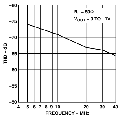
Figure 15. THD vs. Clock Frequency at F_{OUT} = 1 \text{ MHz}
