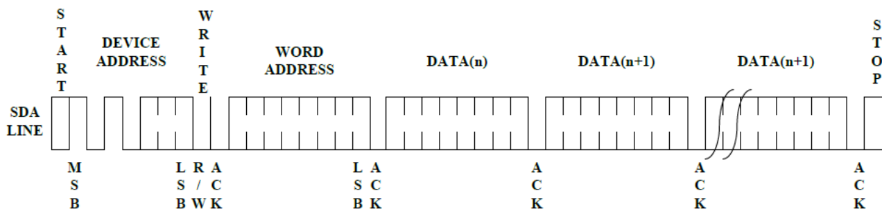
Figure 7 Page Write
