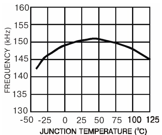
Switching Frequency
