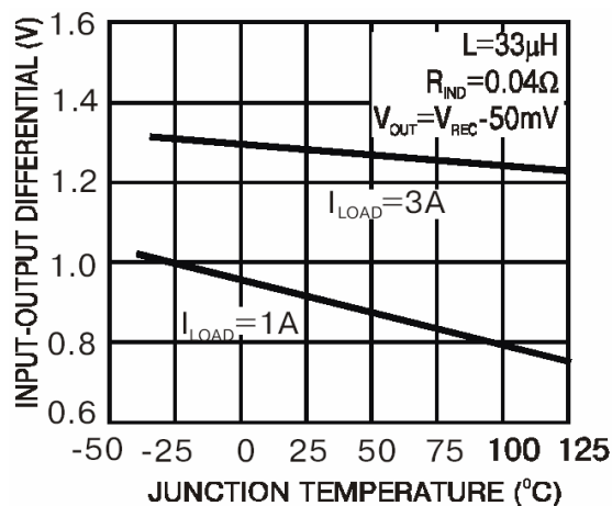
Dropout Voltage
