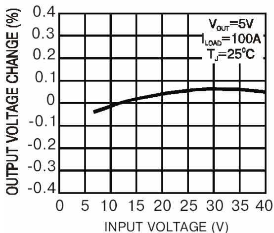
Line Regulator
