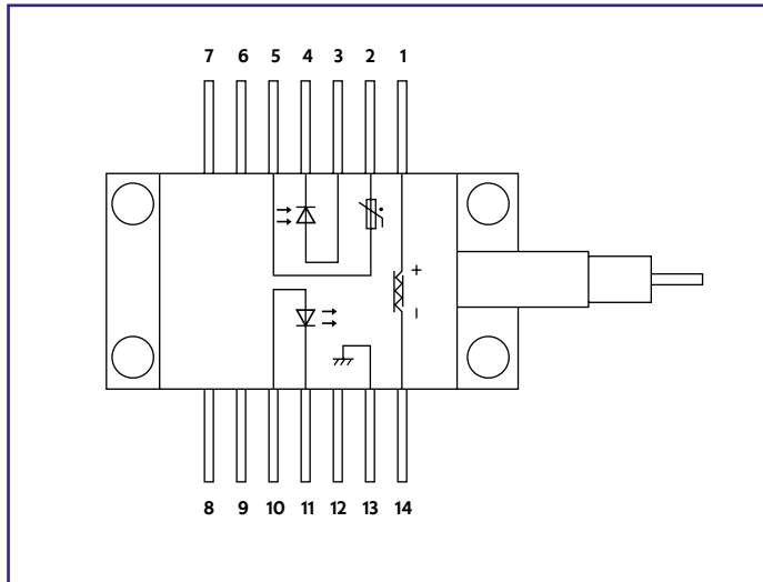
Figure 2: Connections
