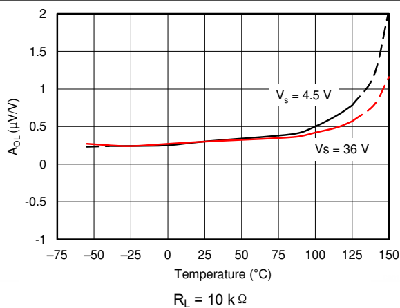
图 7-23. Open-Loop Gain vs Temperature
