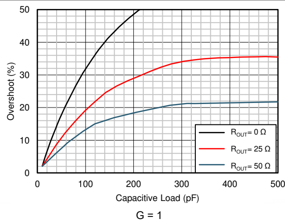
图 8-4. Small-Signal Overshoot vs Capacitive Load (100-mV Output Step)
