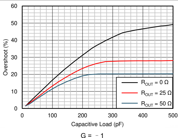
图 8-3. Small-Signal Overshoot vs Capacitive Load (100-mV Output Step)
