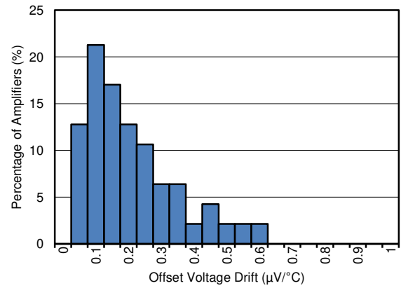
图 7-2. Offset Voltage Drift Production Distribution
