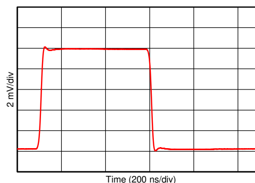
图 7-32. Small-Signal Step Response
