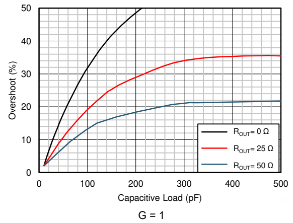
图 7-26. Small-Signal Overshoot vs Capacitive Load (100-mV Output Step)
