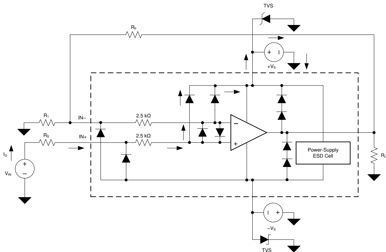
图 8-5. Equivalent Internal ESD Circuitry Relative to a Typical Circuit Application
