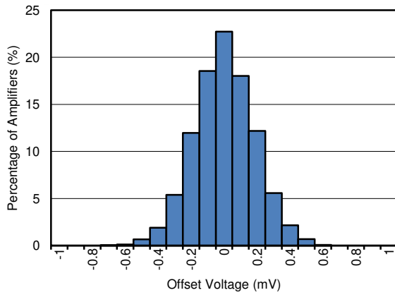
图 7-1. Offset Voltage Production Distribution
