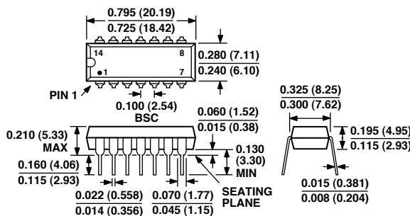
14-Lead Plastic DIP Package (P-Suffix)
