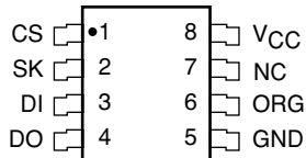
TSSOP Package (U,Y)
