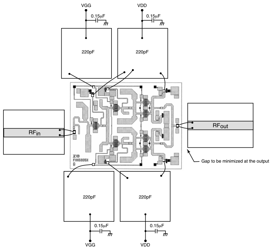
ASSEMBLY DRAWING
