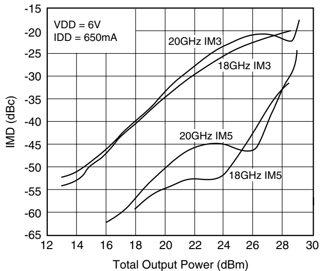
OUTPUT POWER vs. IMD
