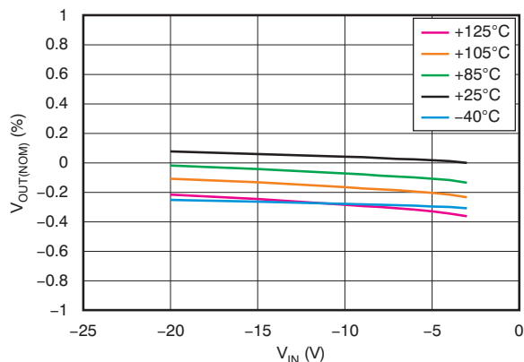
Figure 22. Line Regulation
