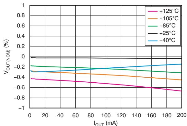
Figure 23. Load Regulation
