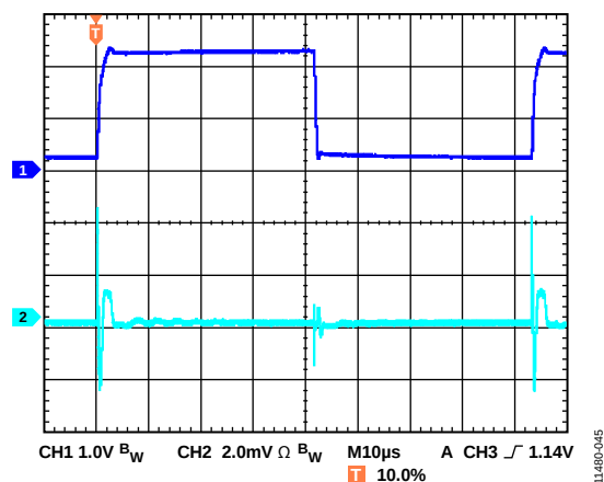
图45. 线路瞬态响应, 2 V输入阶跃, I_{LOAD} = 800\text{ mA} , V_{OUT} = 3.3\text{ V} , V_{IN} = 4.5\text{ V} , CH1 = V_{IN} , CH2 = V_{OUT}
