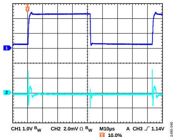
图46. 线路瞬态响应, 2 V输入阶跃, I_{LOAD} = 800\text{ mA} , V_{OUT} = 5\text{ V} , V_{IN} = 6.2\text{ V} , CH1 = V_{IN} , CH2 = V_{OUT}
