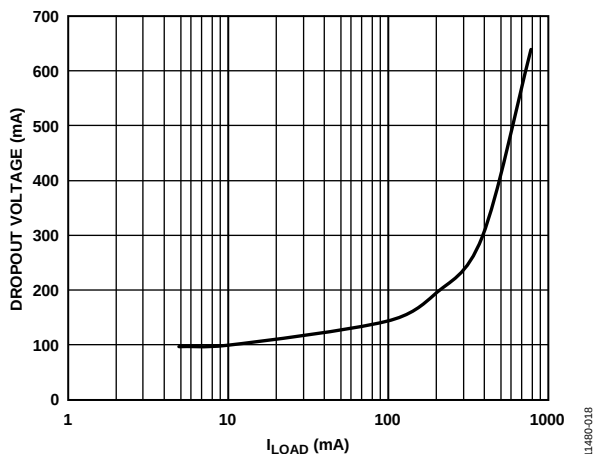
图18. 压差与负载电流( I_{LOAD} )的关系, ADM7151-04, V_{OUT} = 5V
