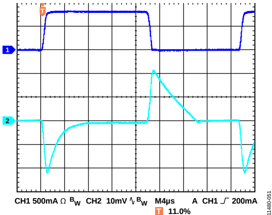
图51. 输出瞬态响应( V_{OUT} = 5\text{ V} , C_{OUT} = 10\text{ }\mu\text{F} )
