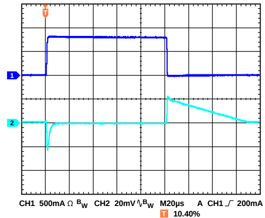
图40. 负载瞬态响应, I_{LOAD} = 1 \text{ mA} 至 800 \text{ mA} , V_{OUT} = 5 \text{ V} , V_{IN} = 6.2 \text{ V} , CH1 = I_{OUT} , CH2 = V_{OUT}
