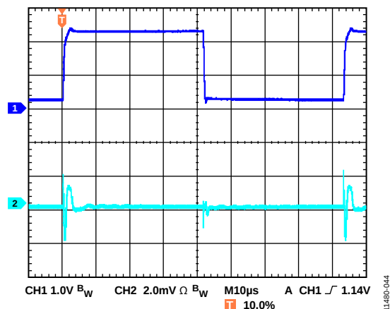
图44. 线路瞬态响应, 2 V输入阶跃, I_{LOAD} = 800\text{ mA} , V_{OUT} = 1.8\text{ V} , V_{IN} = 4.5\text{ V} , CH1 = V_{IN} , CH2 = V_{OUT}
