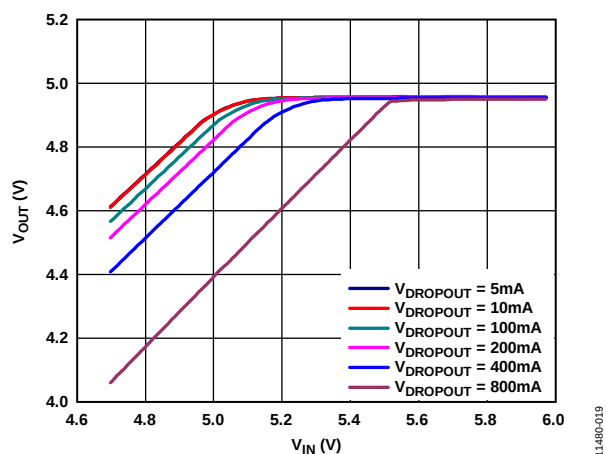
图19. 压差条件下输出电压( V_{OUT} )与输入电压( V_{IN} )的关系, ADM7151-04, V_{OUT} = 5V
