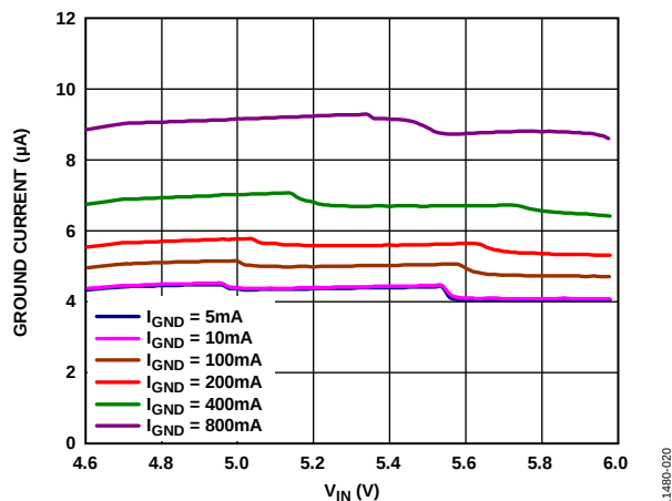
图20. 压差条件下接地电流与输入电压( V_{IN} )的关系, ADM7151-04, V_{OUT} = 5V
