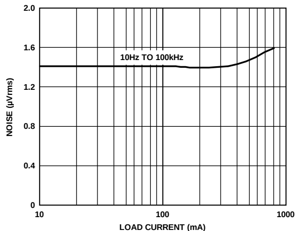
图33. RMS输出噪声与负载电流( I_{LOAD} )的关系, 10 Hz至100 kHz, ADM7151-02, V_{OUT} = 4\text{ V}
