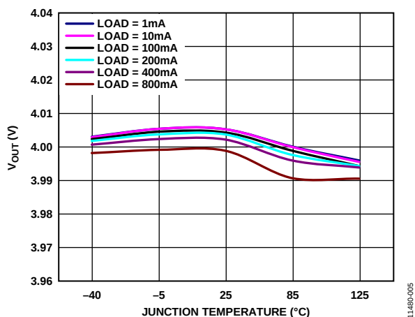
图5. 输出电压( V_{OUT} )与结温( T_J )的关系, ADM7151-02, V_{OUT} = 4\text{ V}
