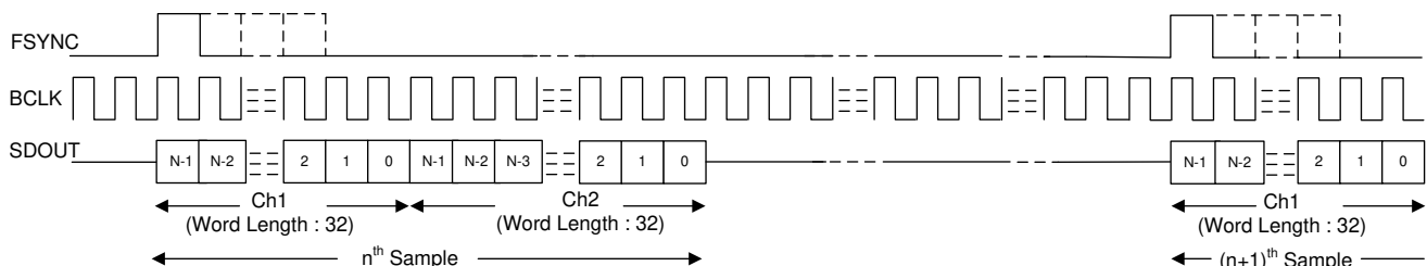
Figure 8-1. TDM Mode Protocol Timing (FMT0 = HIGH) In Slave Mode
