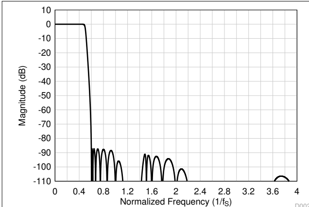
Figure 8-23. Low-Latency Decimation Filter Magnitude Response
