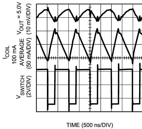
Boost Typical Waveforms at 100 mA Load
