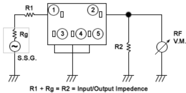
Figure 2) Measuring Circuit
