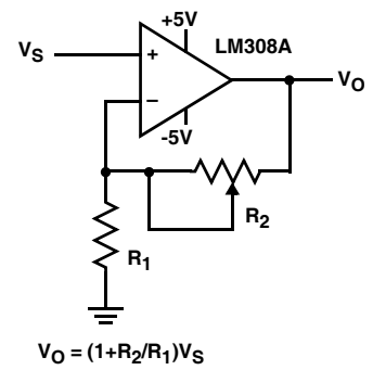
NONINVERTING AMPLIFIER
