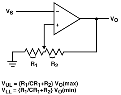
COMPARATOR WITH HYSTERITIS
