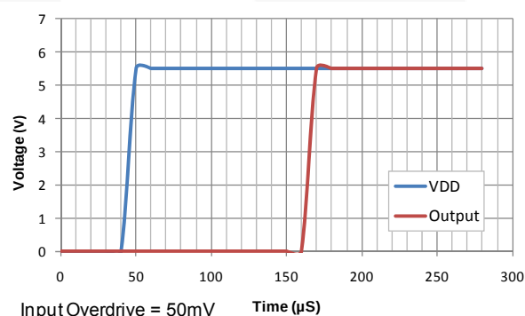
Figure 13. Power-Up Delay
