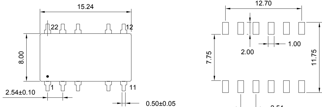
SUGGESTED PAD LAYOUT
