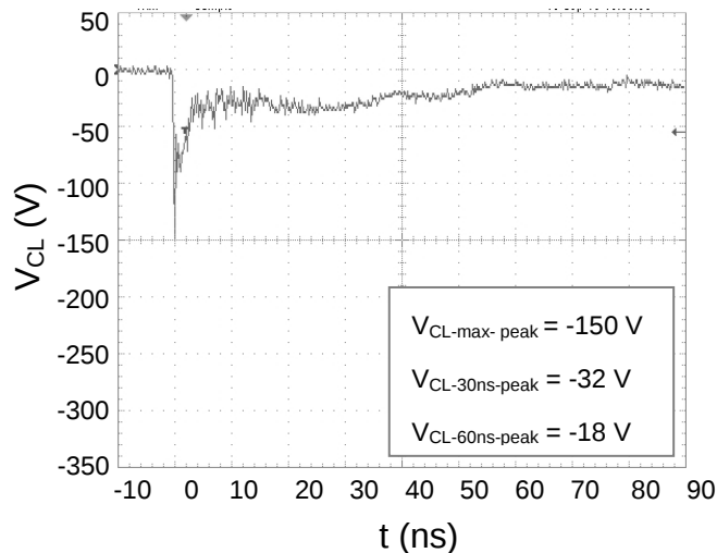
-15kV contact ESD
