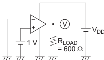
2. Output High Voltage, V_{OH} (Output High)
