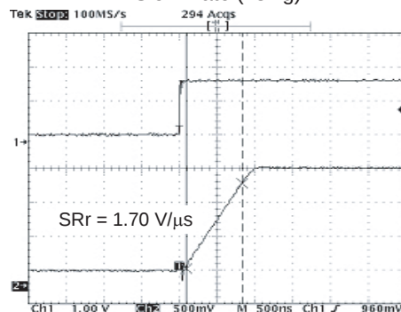
Figure 20 HA1630S08 Slew Rate (rising)
