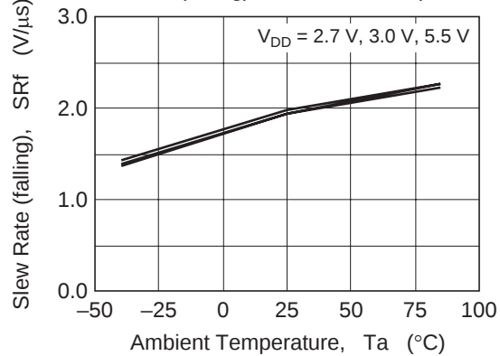
Figure 22 HA1630S08 Slew Rate (falling) vs. Ambient Temperature
