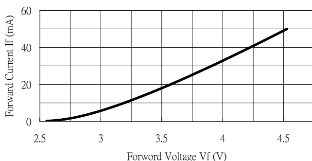
Fig. 2 Forward Current VS Forward Voltage
